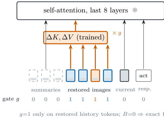
(a) HGKV training
