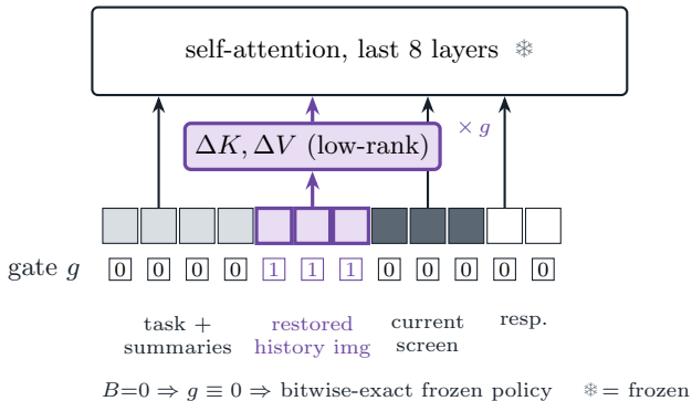
(a) hgkv: gated K/V interface
