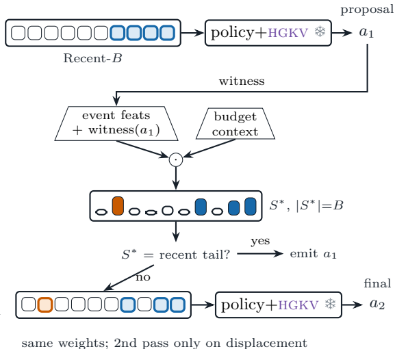
(b) proposal-conditioned re-decision
