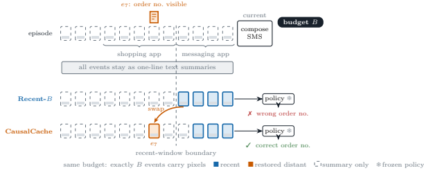
Figure 1: CAUSALCACHE on a real cross-app episode (schematic; drawn with B=4 ). The agent must compose an SMS containing the order number it saw earlier in a shopping app. Every event persists as a one-line text summary; a budget of B events may additionally carry their archived pixels. After the app switch the evidence frame e_7 lies outside the recent window: Recent- B spends every slot on the latest events and types the wrong number, while CAUSALCACHE swaps one recent slot for e_7 at the same budget and succeeds.
