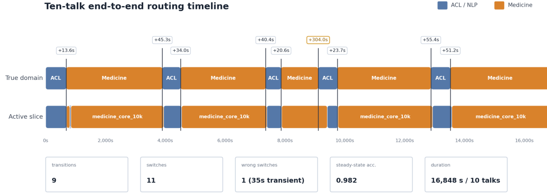
Figure 3: Active-glossary routing over the ten-talk alternating run of Table 1 (16,848s streamed end-to-end through one live session). All nine domain transitions switch in the correct direction; eight land 13.6–55.4s after the boundary and one medicine-to-ACL switch (amber) is delayed 304s over a generic talk opening. A single 35s transient wrong switch self-corrects; steady-state active-domain accuracy is 0.982 outside 30s transition grace windows.
