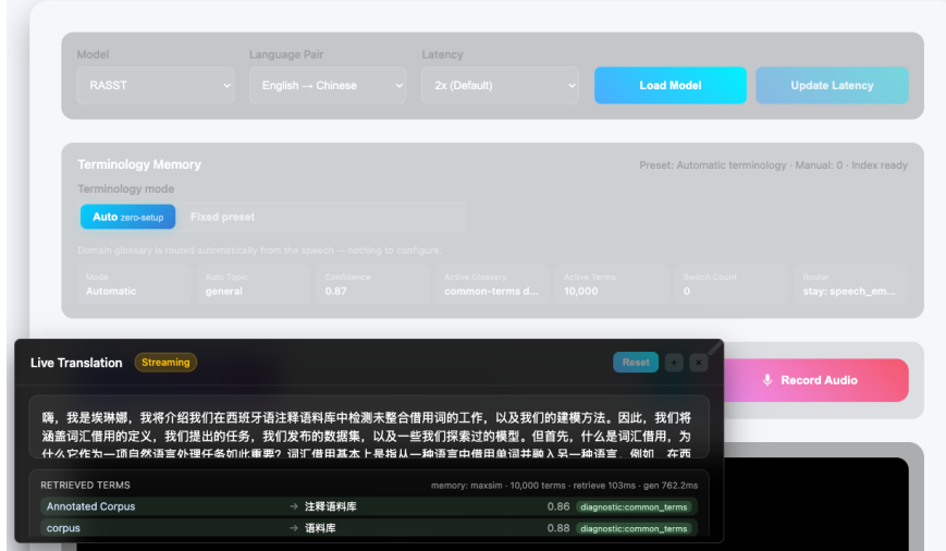
Figure 2: Web UI during a live session. The top row sets language pair, latency multiplier, and terminology mode (Auto or Fixed); the chips and the panel below render the JSON evidence stream: active glossary, router confidence, retrieved term pairs with retrieval scores, and per-chunk retrieval/generation latency. The shown session uses a diagnostic slice; production sessions start from domain slices.
