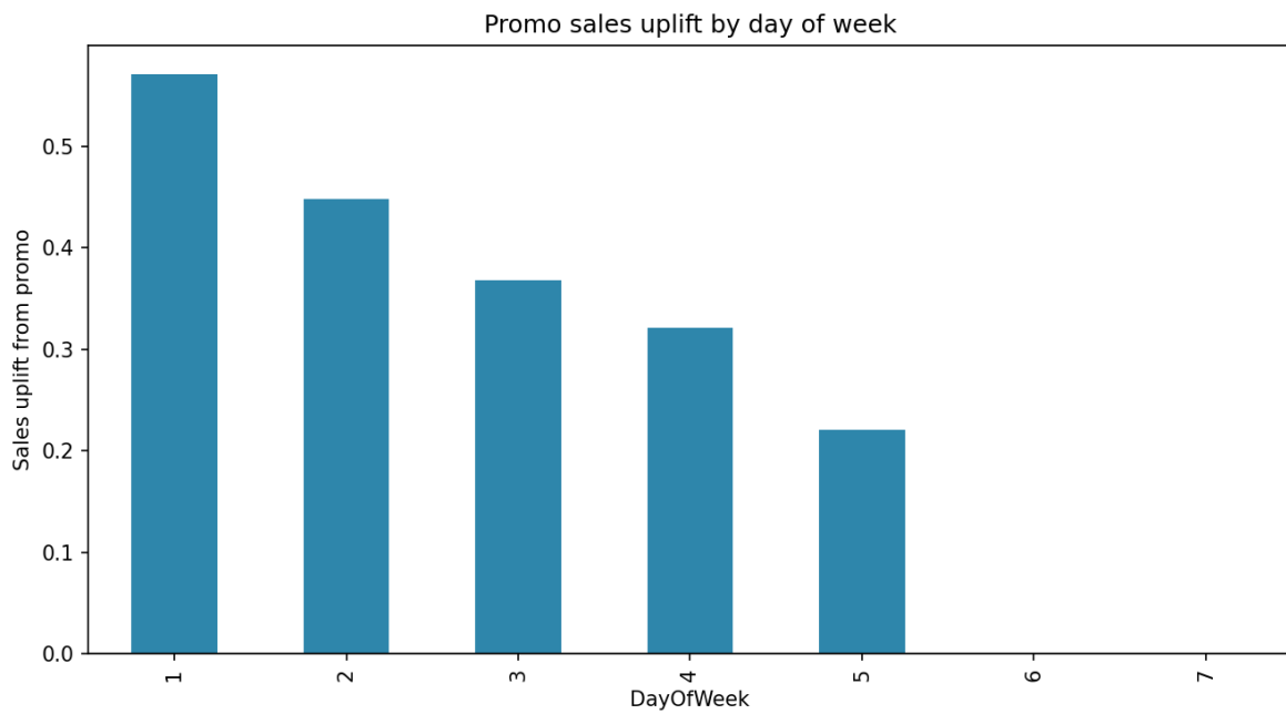
Fig 1. Promo sales uplift by day of week — decays from Monday to Friday.
