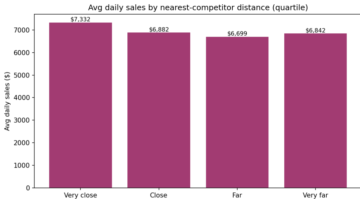
Fig 2. Avg daily sales by nearest-competitor distance — no meaningful penalty for proximity.
