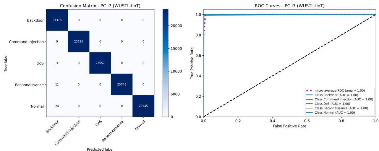
Fig. 10. Confusion matrix and ROC of WUSTL-IIoT on PC (i7).
