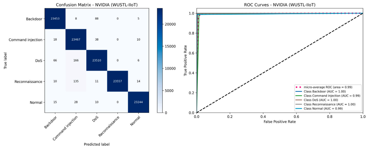
Fig. 12. Confusion matrix and ROC of WUSTL-IIoT on NVIDIA.
