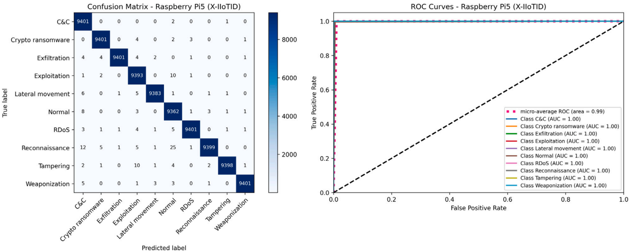
Fig. 8. Confusion matrix and ROC of X-IloTID on Raspberry (Pi 5).
