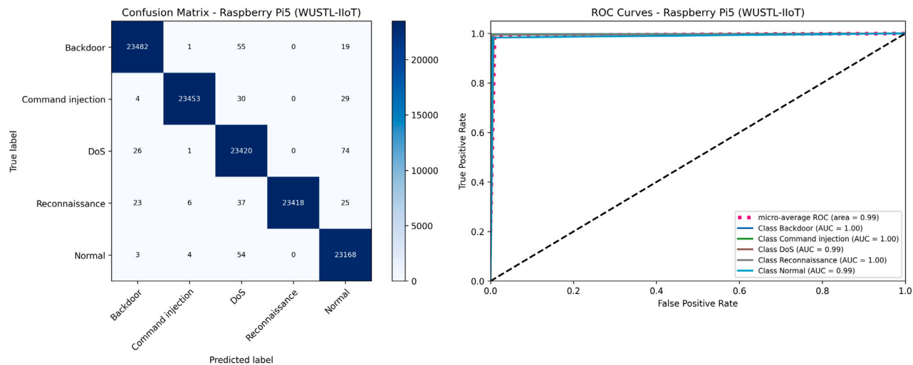
Fig. 11. Confusion matrix and ROC of WUSTL-IIoT on Raspberry (Pi 5).
