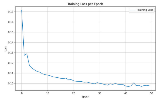
Fig. 5. Loss per epoch of X-IIoTID.
