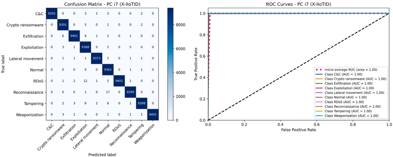
Fig. 7. Confusion matrix and ROC of X-IloTID on PC (i7).
