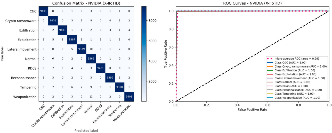
Fig. 9. Confusion matrix and ROC of X-IloTID on NVIDIA.
