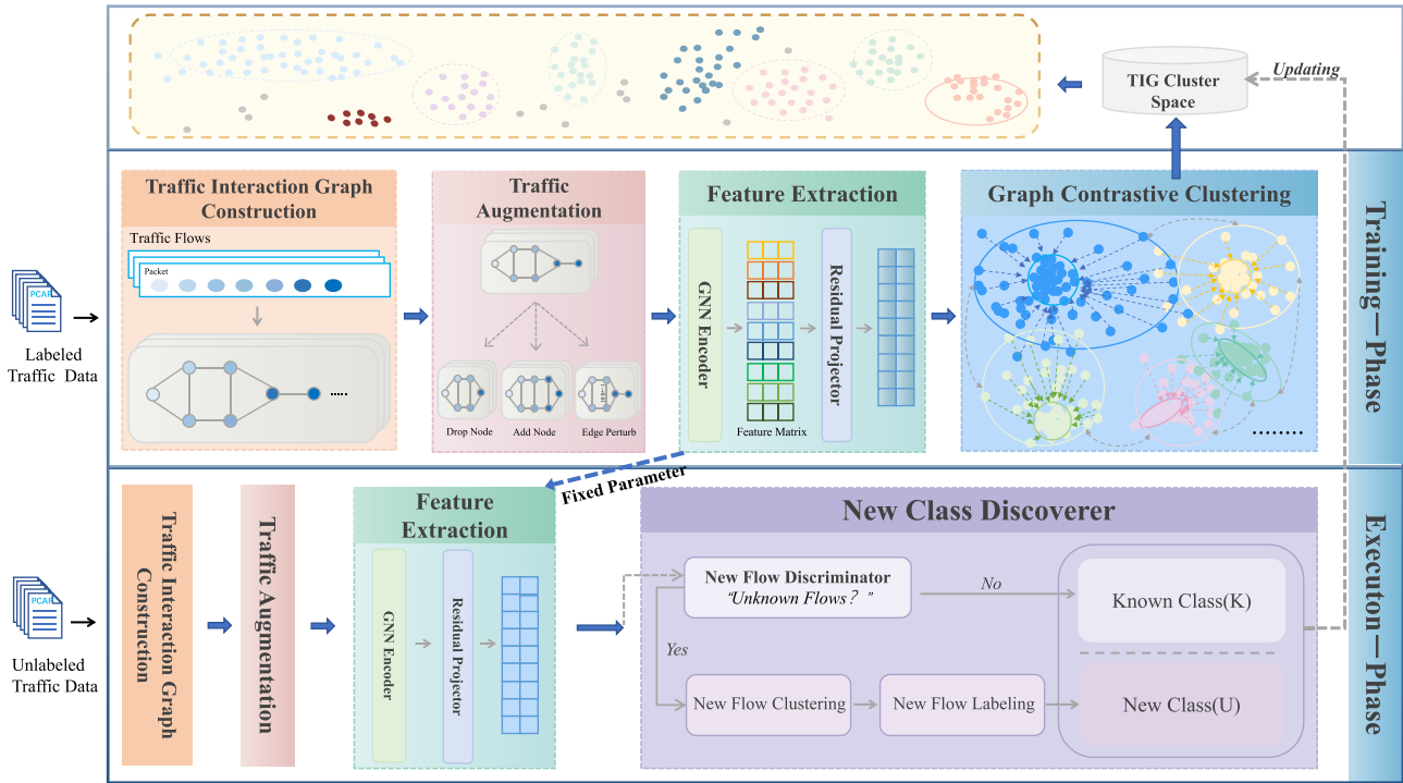
Fig. 2. Overview of the proposed GCLC framework. During training, labeled traffic graphs are used in supervised contrastive clustering to form distinct class clusters. During execution, new flows are embedded and compared against known clusters for classification or new class detection.
