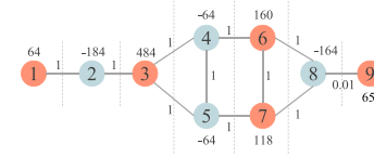
Fig. 4. Traffic interaction graph (TIG) for flows.
