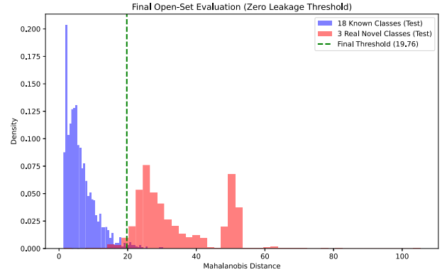
Fig. 12. Density distributions of Mahalanobis distances for known (blue) and novel (red) classes, with the zero-leakage threshold at 19.76 marked by the green dashed line.
