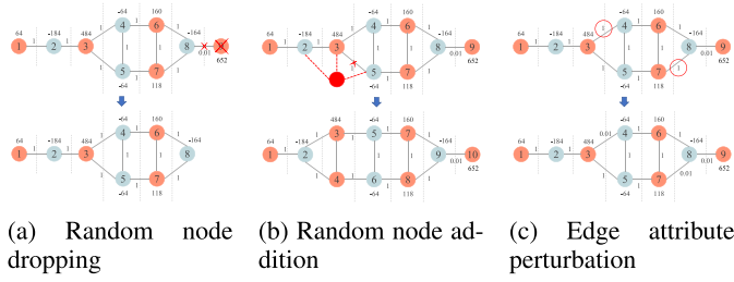
Fig. 5. Illustration of various network traffic perturbations: (a) Random node dropping, (b) Random node addition, and (c) Edge attribute perturbation.
