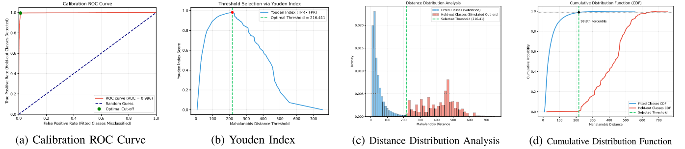
Fig. 11. Threshold selection via ROC and distance distribution analysis, showing clear separation between fitted and hold-out classes.
