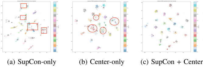
Fig. 9. Ablation t-SNE on APPLICATIONS_21: combining SupCon and Center-aware losses produces the most compact and clearly separated clusters.
