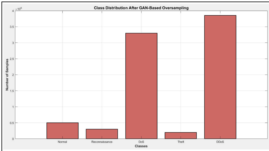
Fig. 6. Class-wise sample distribution after GAN-based oversampling for Bot-IoT dataset.
