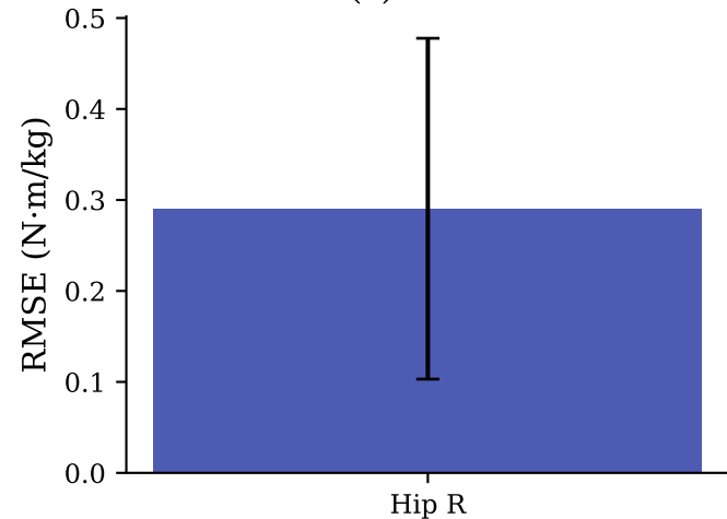
(a) RMSE
