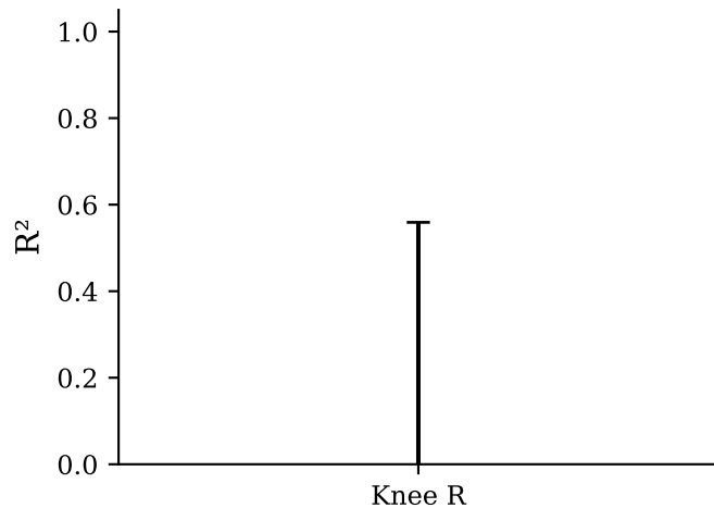
(b) R^2
