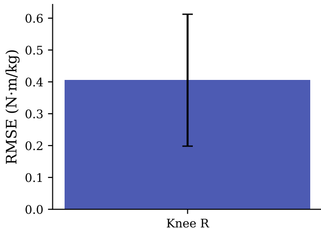
(a) RMSE
