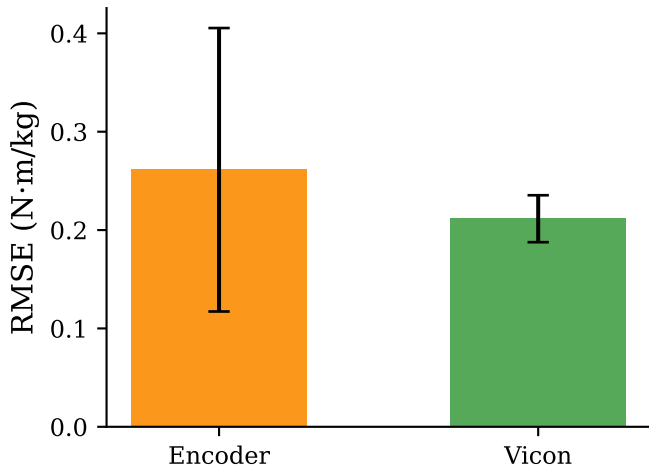
(a) RMSE
