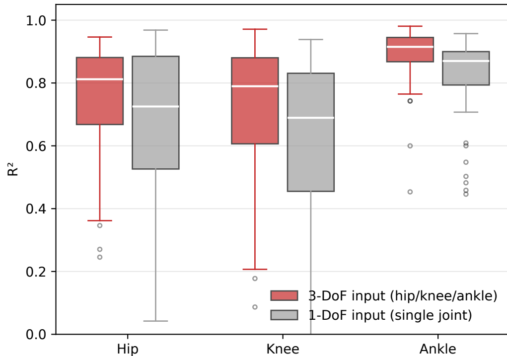
R^2 distribution
