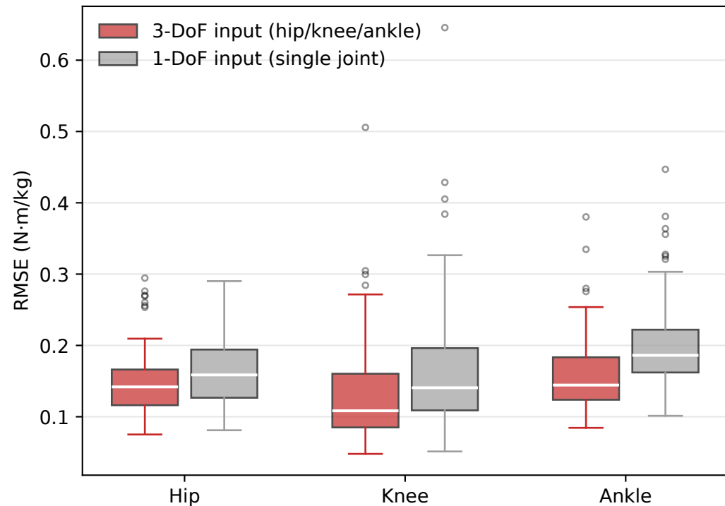
RMSE distribution
