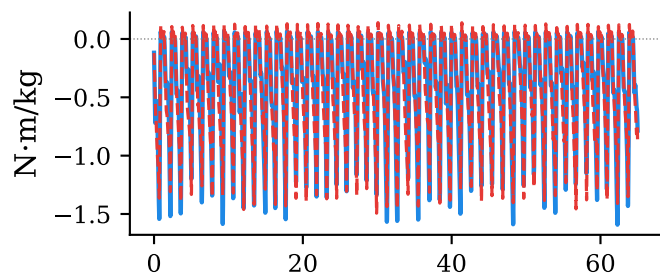
Ankle L R^2=0.90
