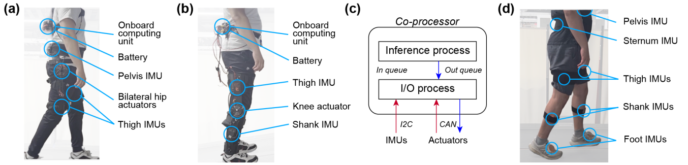
Fig. S1. Overview of the wearable systems and embedded computing architecture used in this study. (a) Bilateral robotic hip exoskeleton, including the onboard computing unit, battery, pelvis IMU, bilateral hip actuators, and thigh IMUs. (b) Robotic knee exoskeleton configuration used during data collection, including the onboard computing unit, battery, thigh IMU, knee actuator, and shank IMU. (c) Embedded co-processor architecture. Separate inference and input/output processes exchange data through input and output queues. IMU measurements are received through I 2 C, and actuator commands are transmitted through CAN. (d) Placement of the sternum, pelvis, bilateral thigh, bilateral shank, and bilateral foot IMUs in the Xsens Awinda sensor suite.
