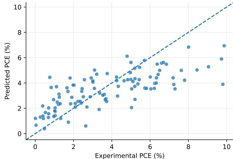
(c) Calibration intercept=-0.7318, slope=1.2975
