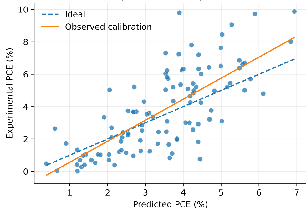
(c) Calibration intercept=-0.7318, slope=1.2975
