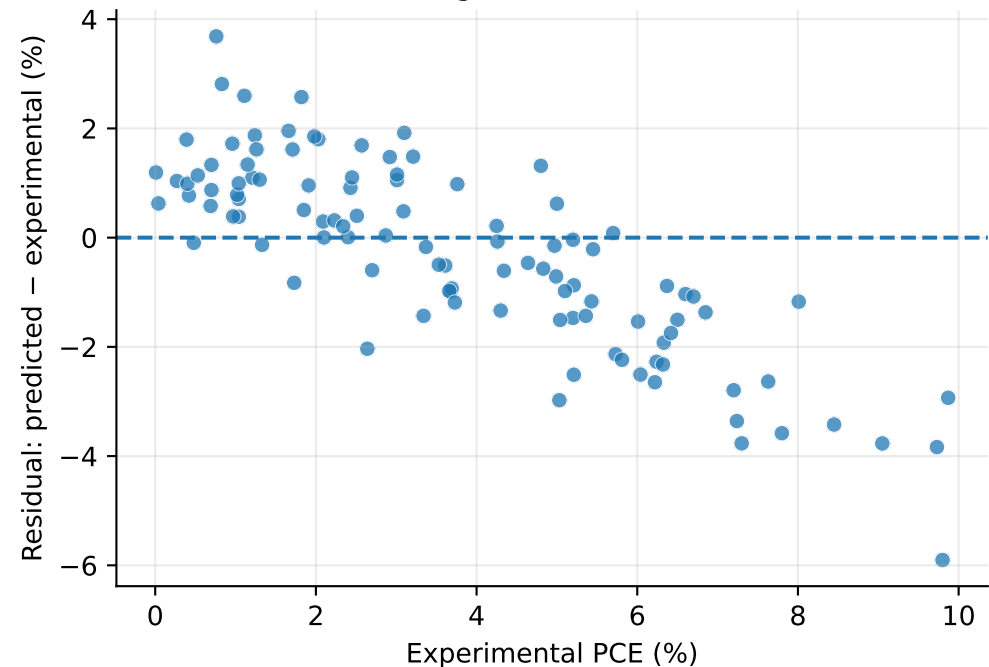
(b) Residual pattern Mean signed error=-0.2934
