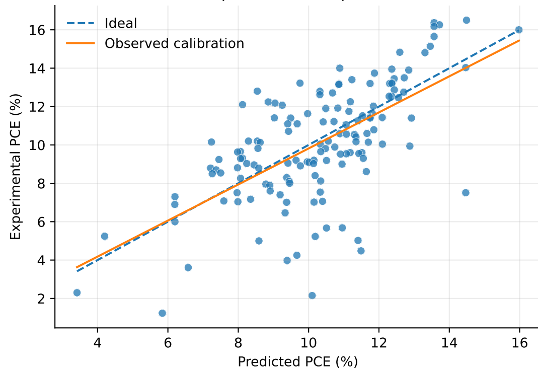
(c) Calibration intercept=0.4209, slope=0.9396
