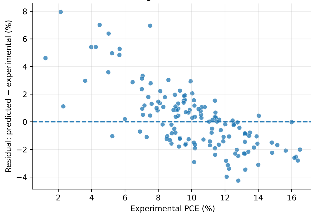
(b) Residual pattern Mean signed error=0.2006
