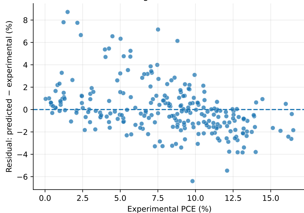
(b) Residual pattern Mean signed error=0.0485
