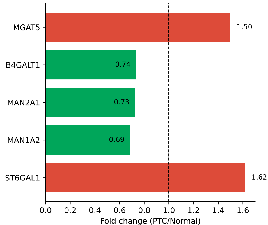
C. 糖基化 (Bones 2018, TCGA)
