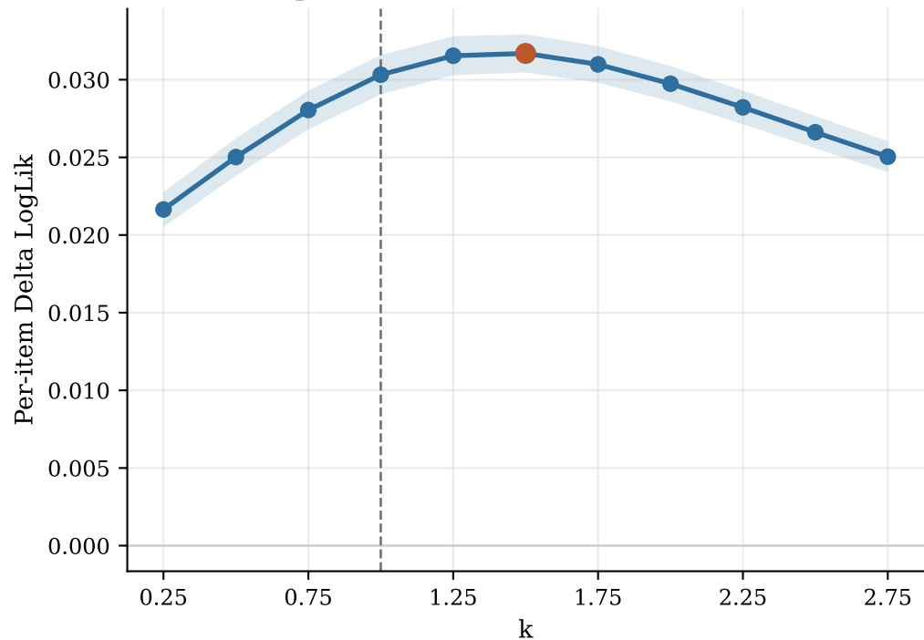
CV Improvement over Verb/Frame Baseline
