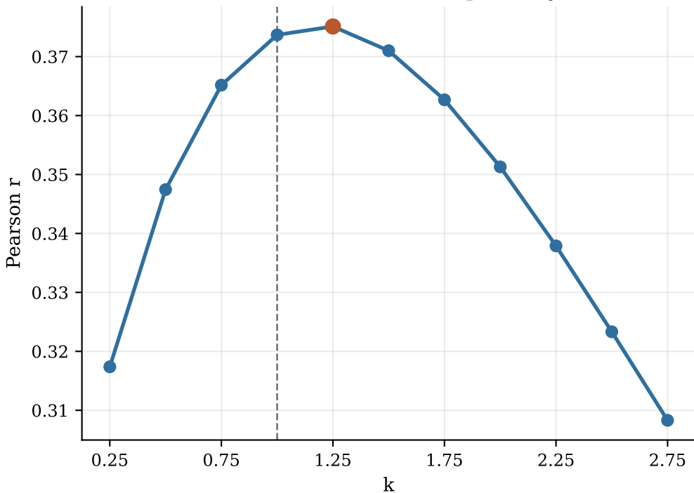
Correlation with Acceptability
