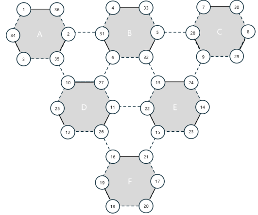
Figure 1: Primal geometric configuration of the lattice gauge model establishing the initial polar boundary invariants.
