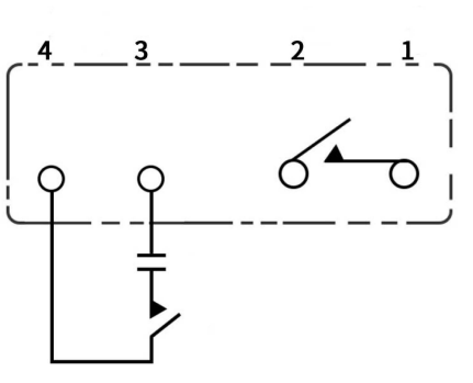
端子配列 (BOTTOM VIEW)
