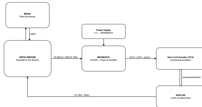
Figure 3.4 BlockdiagramMeasurementSetup
