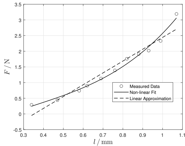
Figure 3.5 SpringTest
