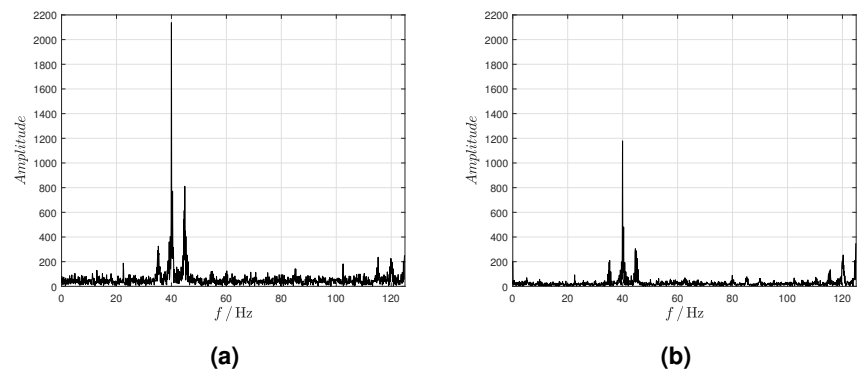
Figure 3.7 (a) With 36g Mass (b) Without Mass
