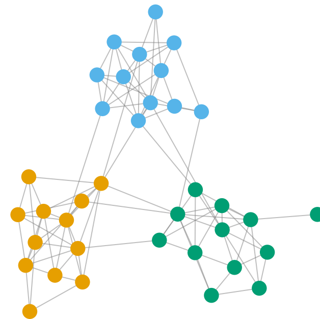
GraphOpt
