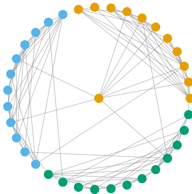
Zvezdasti raspored
