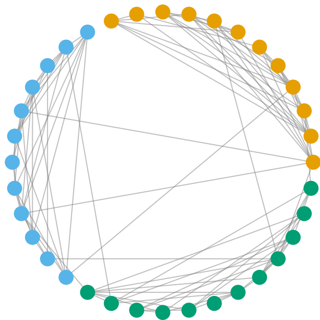
Kružni raspored
