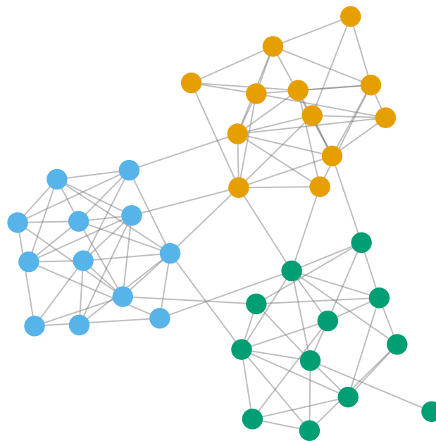
Kamada-Kawai
