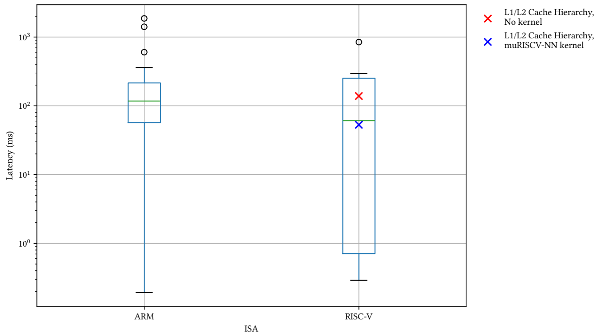
Figure 1: Box Plot of Latency In Inference Application of MobileNetV1in (Visual Wake Words (VWW)) MLPerf Inference Tiny (Lower Is Better)
