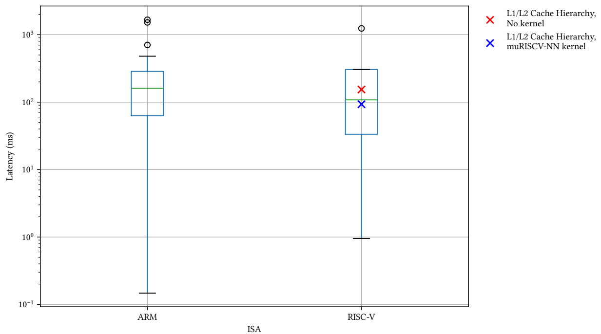
Figure 2: Box Plot of Latency In Inference Application of ResNet-V1 (Image Classification (IC)) in MLPerf Inference Tiny (Lower Is Better),
