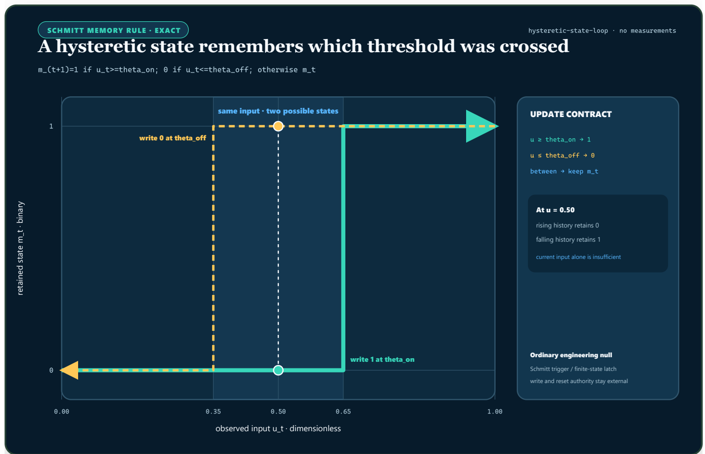
FIGURE 70 — For a binary Schmitt rule, rising and falling input histories form a loop; an input inside the threshold band is compatible with either retained state.
