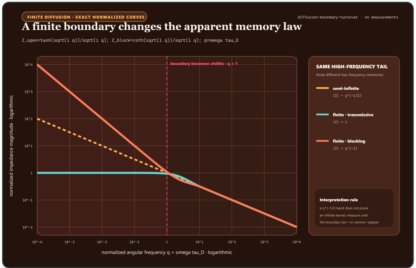
FIGURE 69 – A semi-infinite diffusion law and two finite-boundary laws coincide in their high-frequency slope but separate below the boundary timescale.
