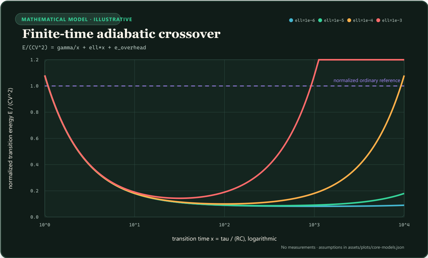
FIGURE 65 — Four normalized adiabatic energy curves form different U-shaped crossovers as leakage changes.
