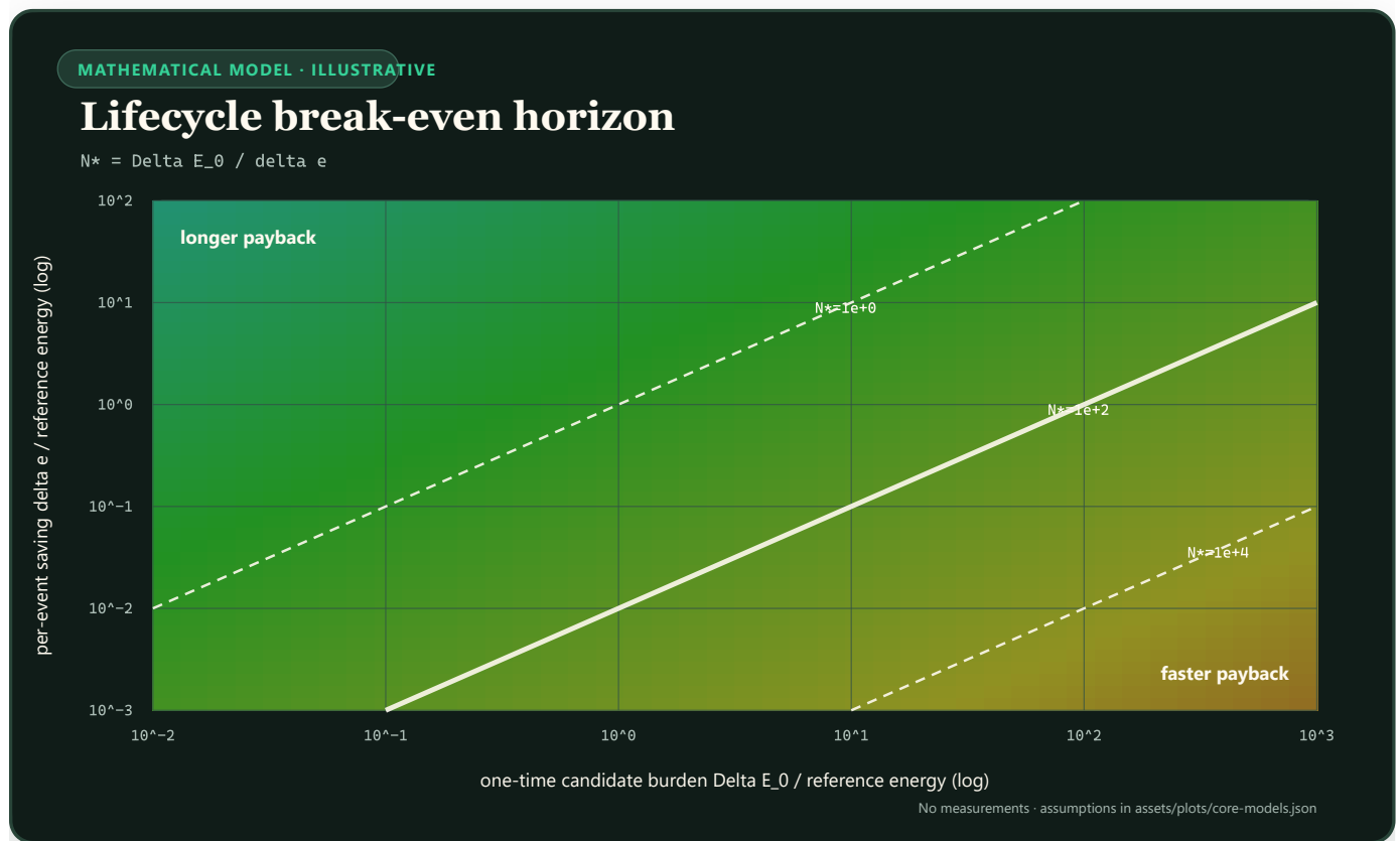
FIGURE 67 — A logarithmic heatmap shows the event count needed to repay one-time candidate burden at different per-event savings.
