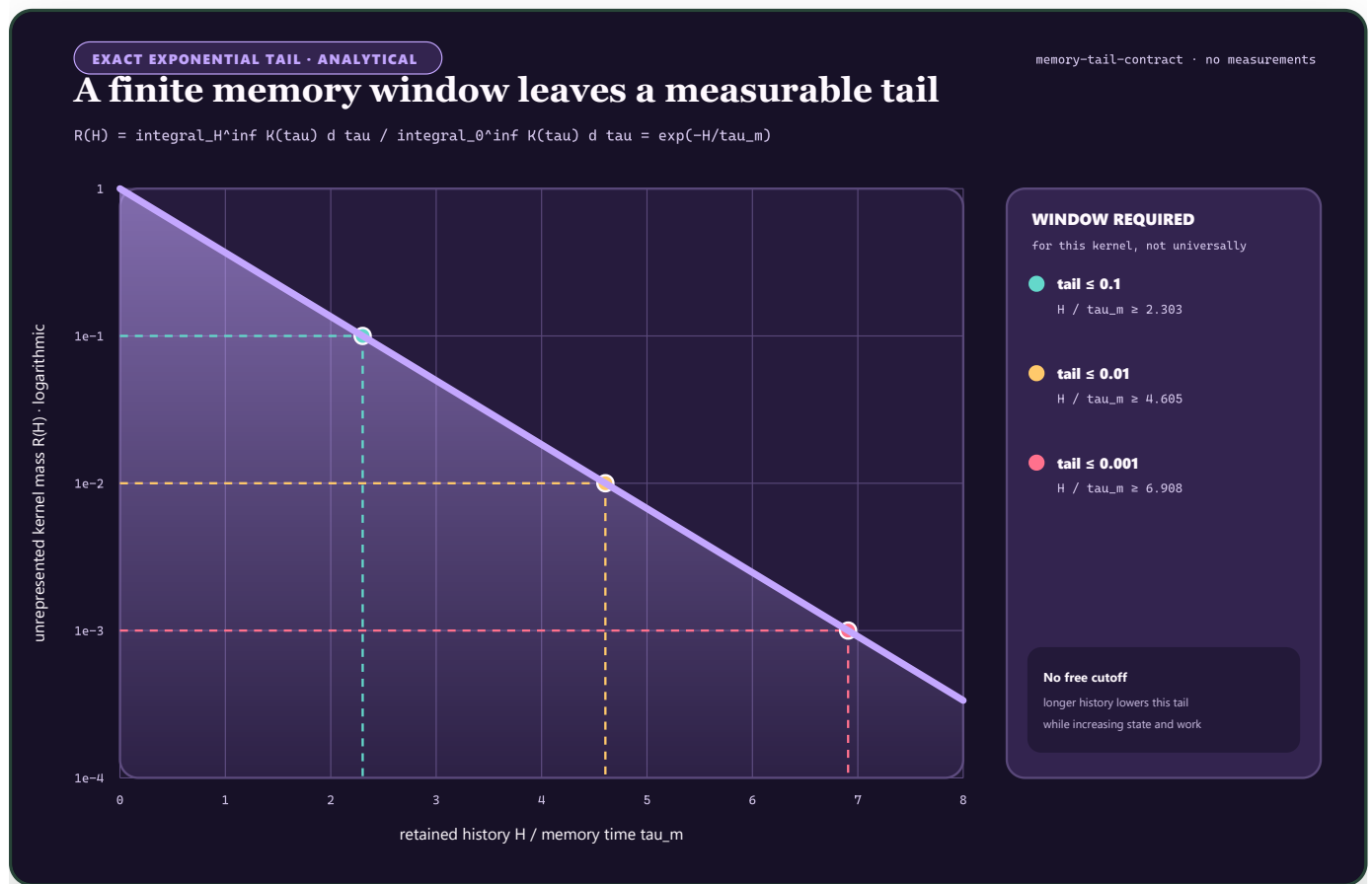
FIGURE 68 — For an exponential memory kernel, the unrepresented tail falls exponentially while every tighter tolerance requires a longer retained history.
