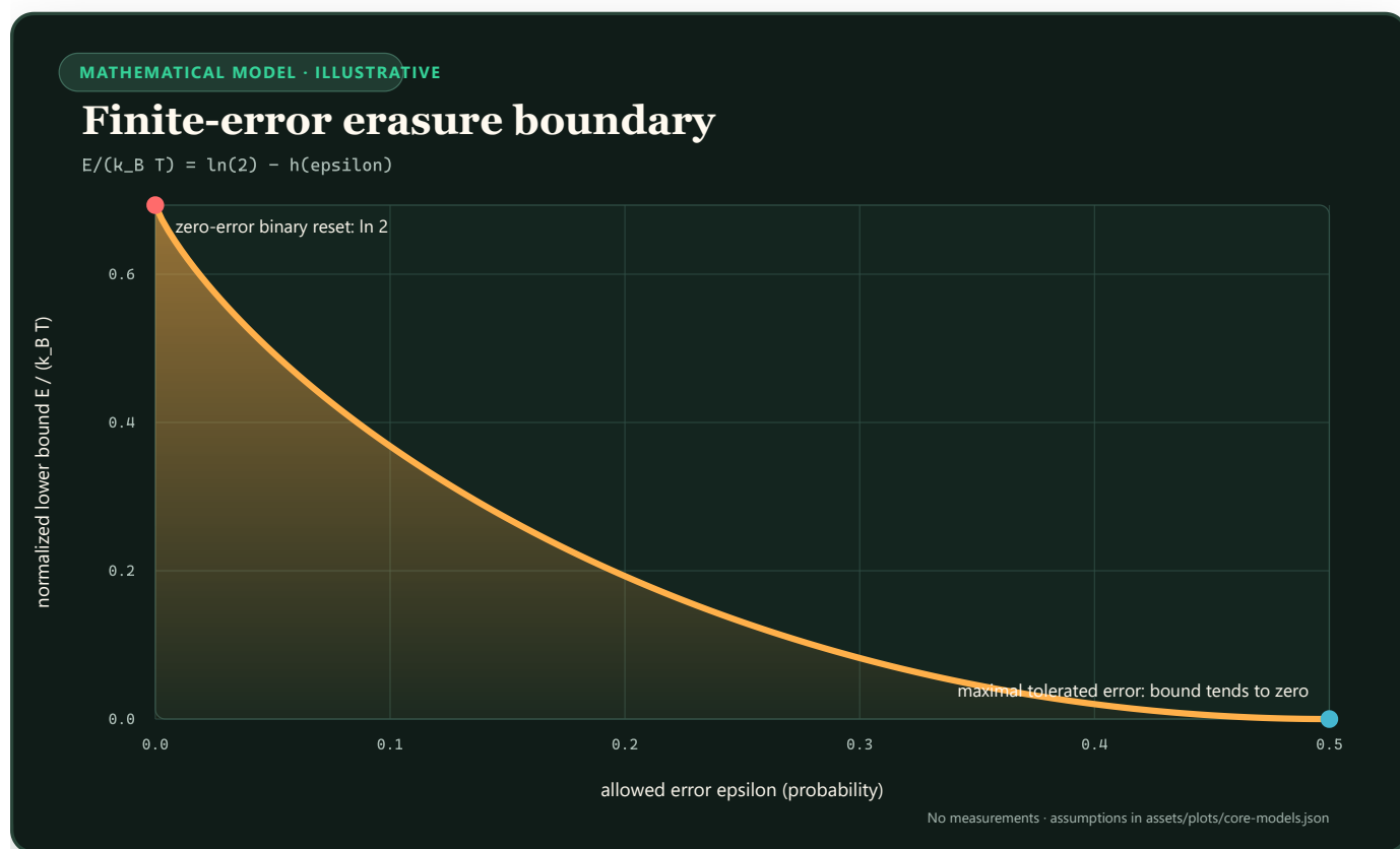
FIGURE 64 — The normalized generalized erasure lower bound falls from \ln 2 at zero error to zero at one-half allowed error.
