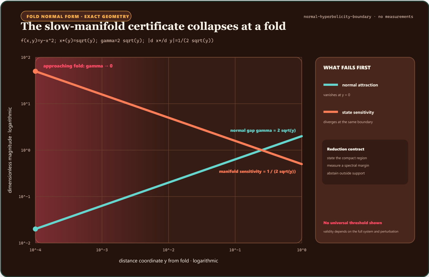
FIGURE 71 – In the fold normal form, the attracting spectral gap falls to zero while the slow-state sensitivity diverges.
