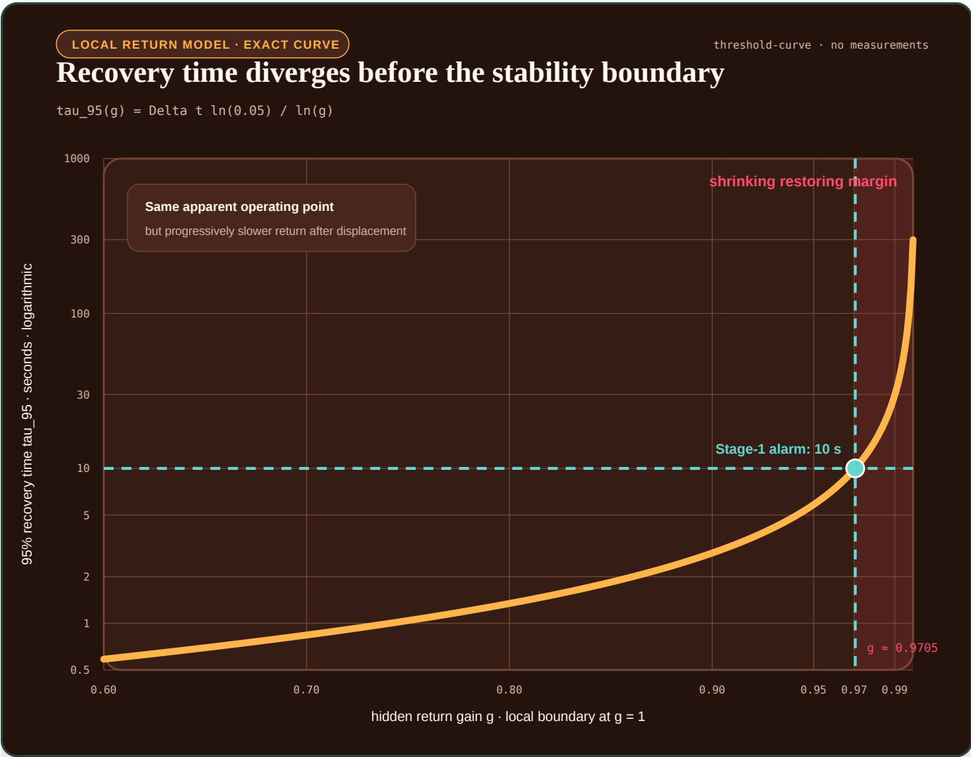
FIGURE 43 – The operating point can look unchanged while recovery time diverges as the local return gain approaches one; the ten-second line is a Stage-1 engineering threshold rather than a biological constant or predicted failure date.
