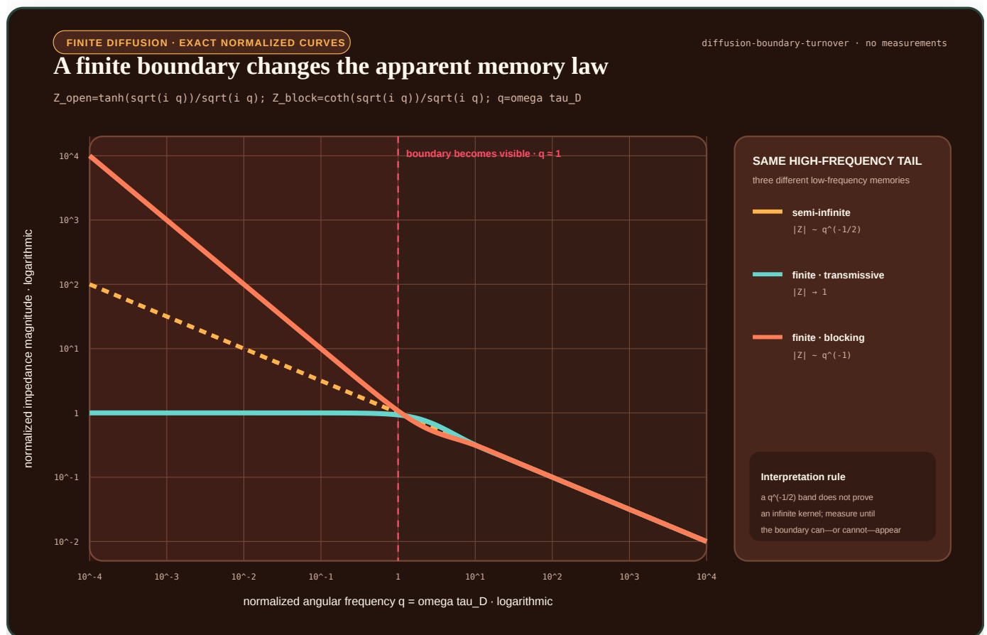
FIGURE 37 — Three normalized diffusion impedances share a high-frequency tail but split into transmissive, blocking, and semi-infinite low-frequency behavior when the boundary becomes observable.
