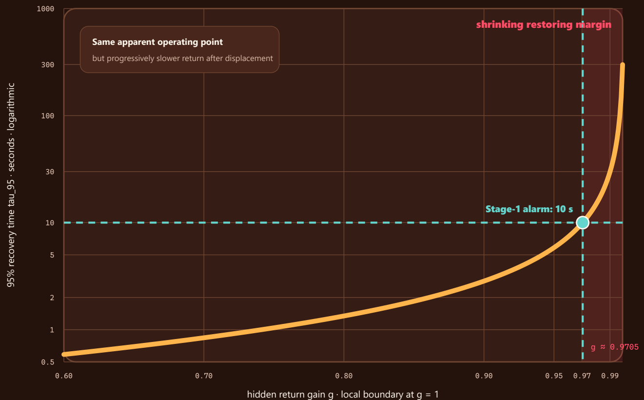
FIGURE 40 — The operating point can look unchanged while recovery time diverges as the local return gain approaches one; the ten-second line is a Stage-1 engineering threshold rather than a biological constant or predicted failure date.
