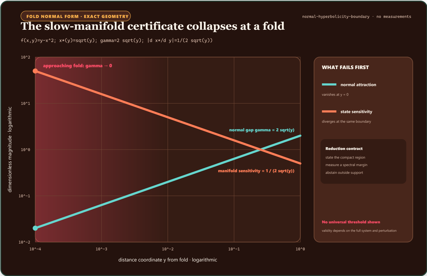
FIGURE 63 – In the fold normal form, the attracting spectral gap falls to zero while the slow-state sensitivity diverges.
