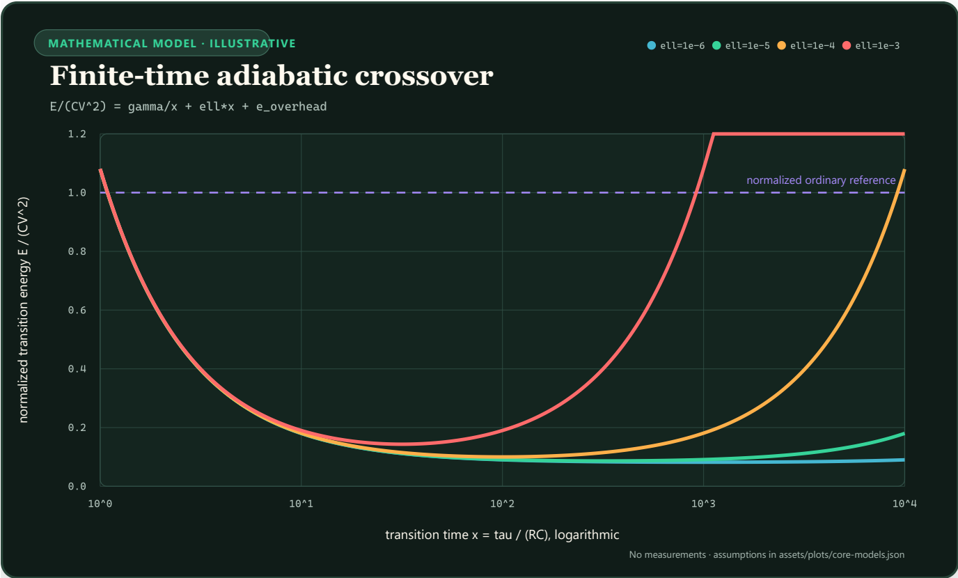
FIGURE 59 — Four normalized adiabatic energy curves form different U-shaped crossovers as leakage changes.
