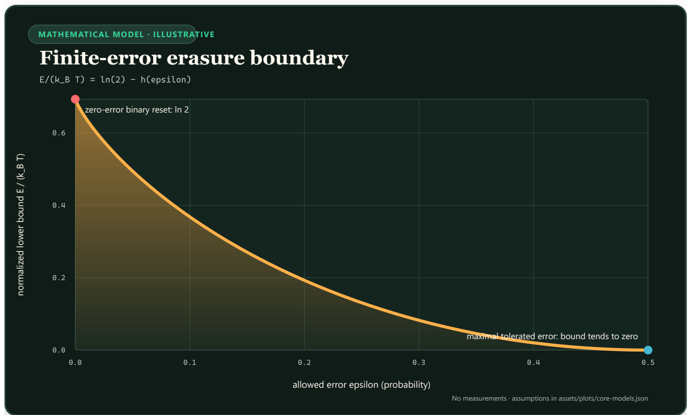
FIGURE 58 — The normalized generalized erasure lower bound falls from \ln 2 at zero error to zero at one-half allowed error.
