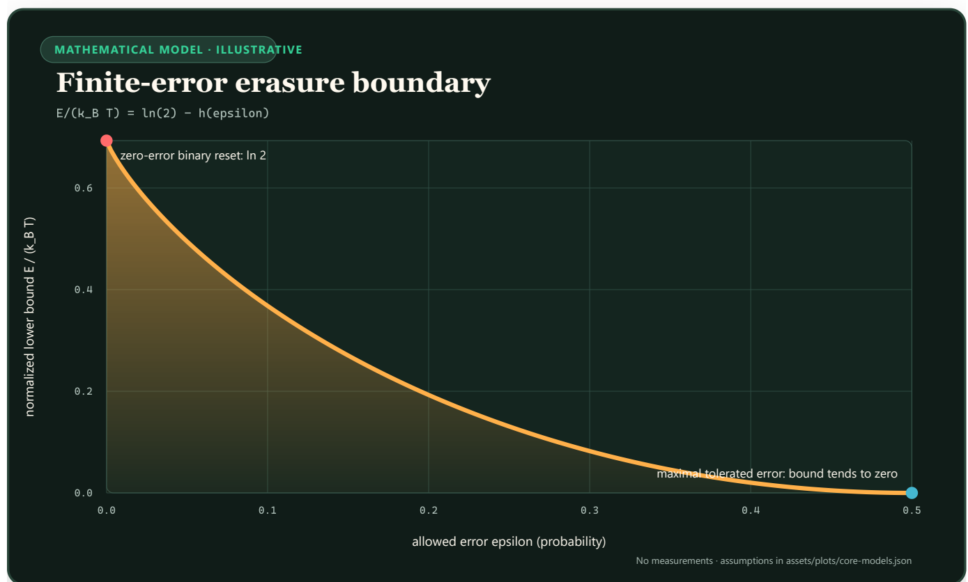
FIGURE 70 — The normalized generalized erasure lower bound falls from \ln 2 at zero error to zero at one-half allowed error.
