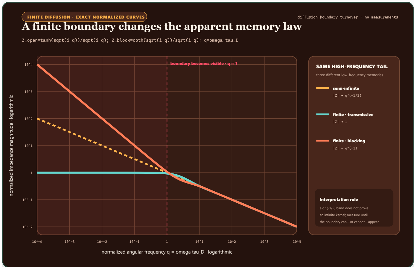
FIGURE 75 – A semi-infinite diffusion law and two finite-boundary laws coincide in their high-frequency slope but separate below the boundary timescale.
