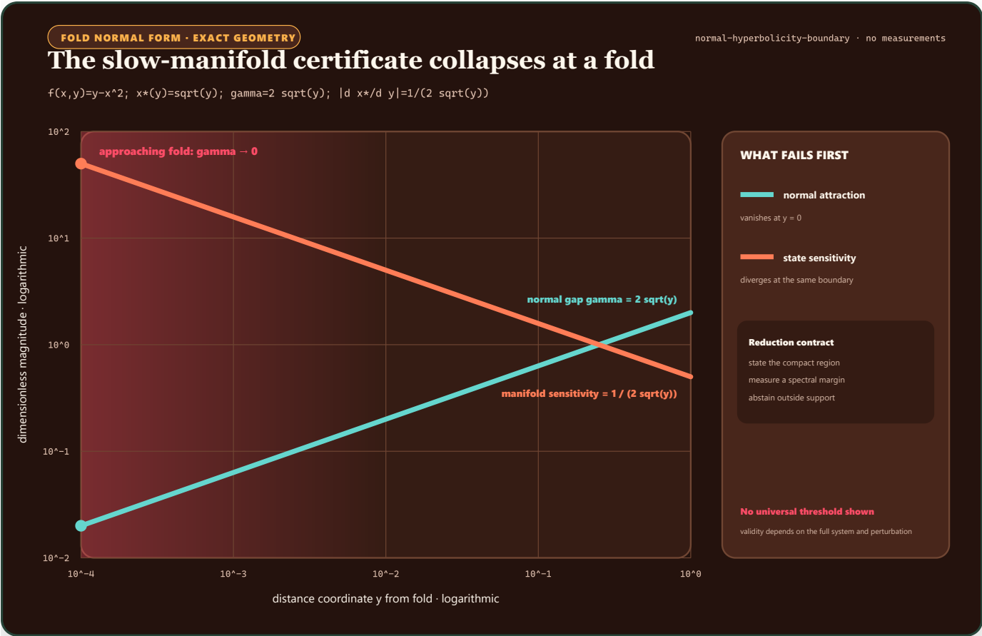
FIGURE 77 – In the fold normal form, the attracting spectral gap falls to zero while the slow-state sensitivity diverges.
