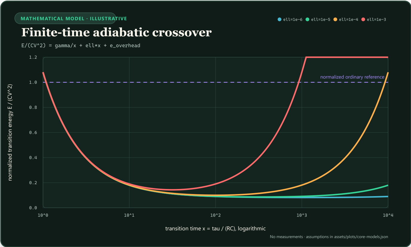
FIGURE 71 — Four normalized adiabatic energy curves form different U-shaped crossovers as leakage changes.
