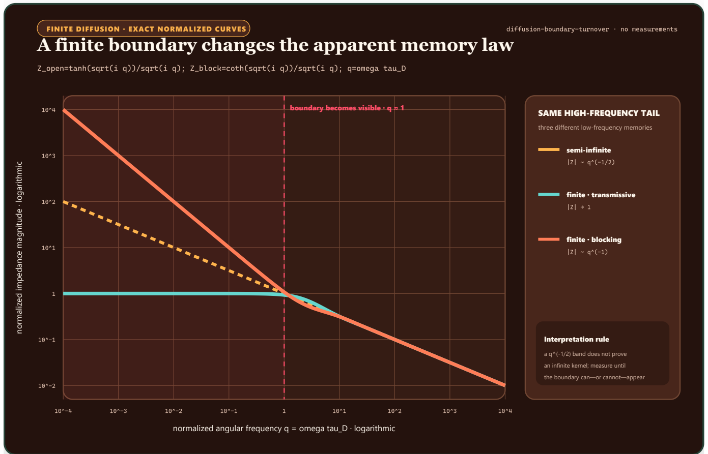
FIGURE 67 – A semi-infinite diffusion law and two finite-boundary laws coincide in their high-frequency slope but separate below the boundary timescale.
