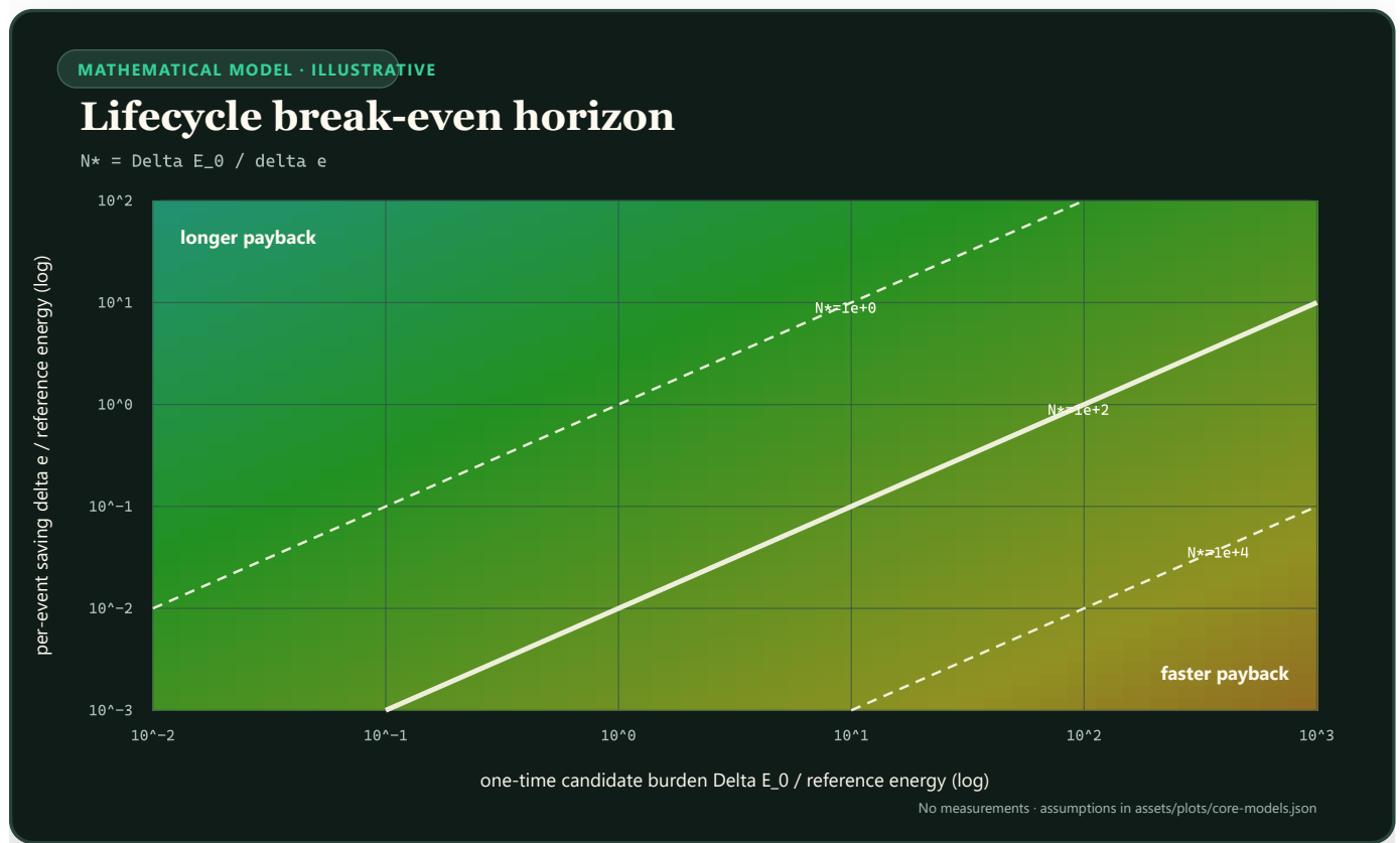
FIGURE 65 — A logarithmic heatmap shows the event count needed to repay one-time candidate burden at different per-event savings.
