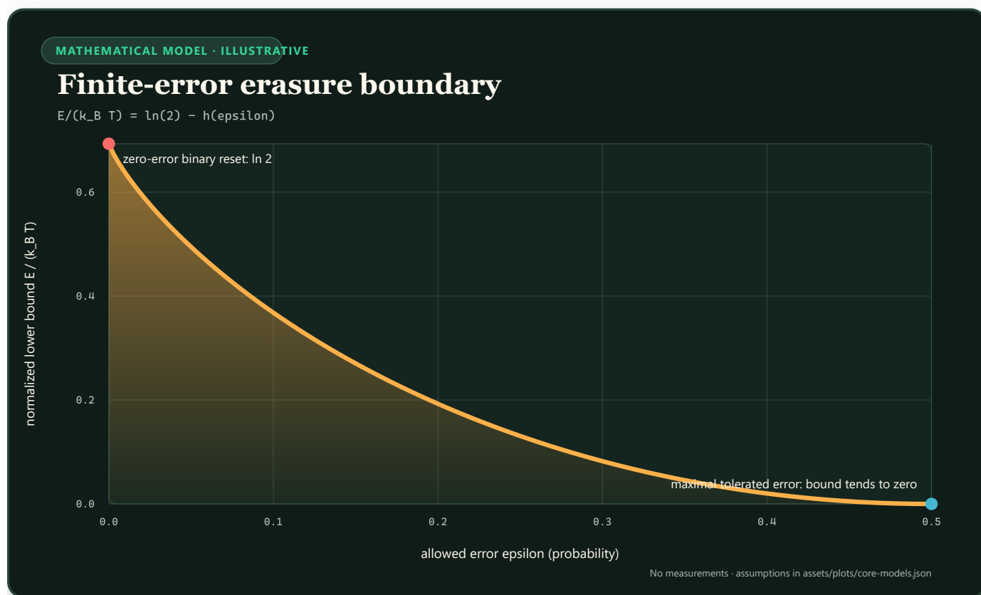
FIGURE 62 — The normalized generalized erasure lower bound falls from \ln 2 at zero error to zero at one-half allowed error.
