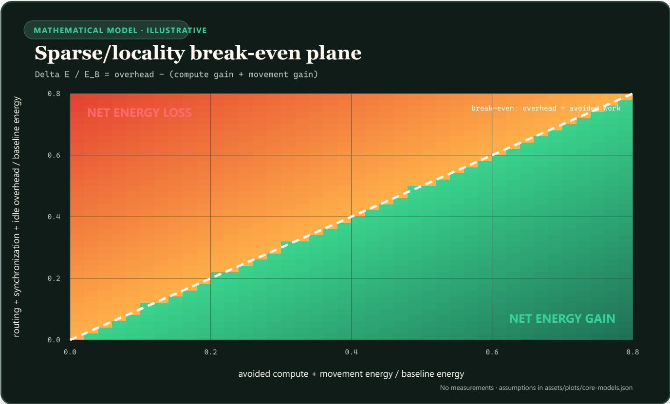
FIGURE 64 — A two-color break-even plane separates net energy gain from net loss at the line where overhead equals avoided work.
