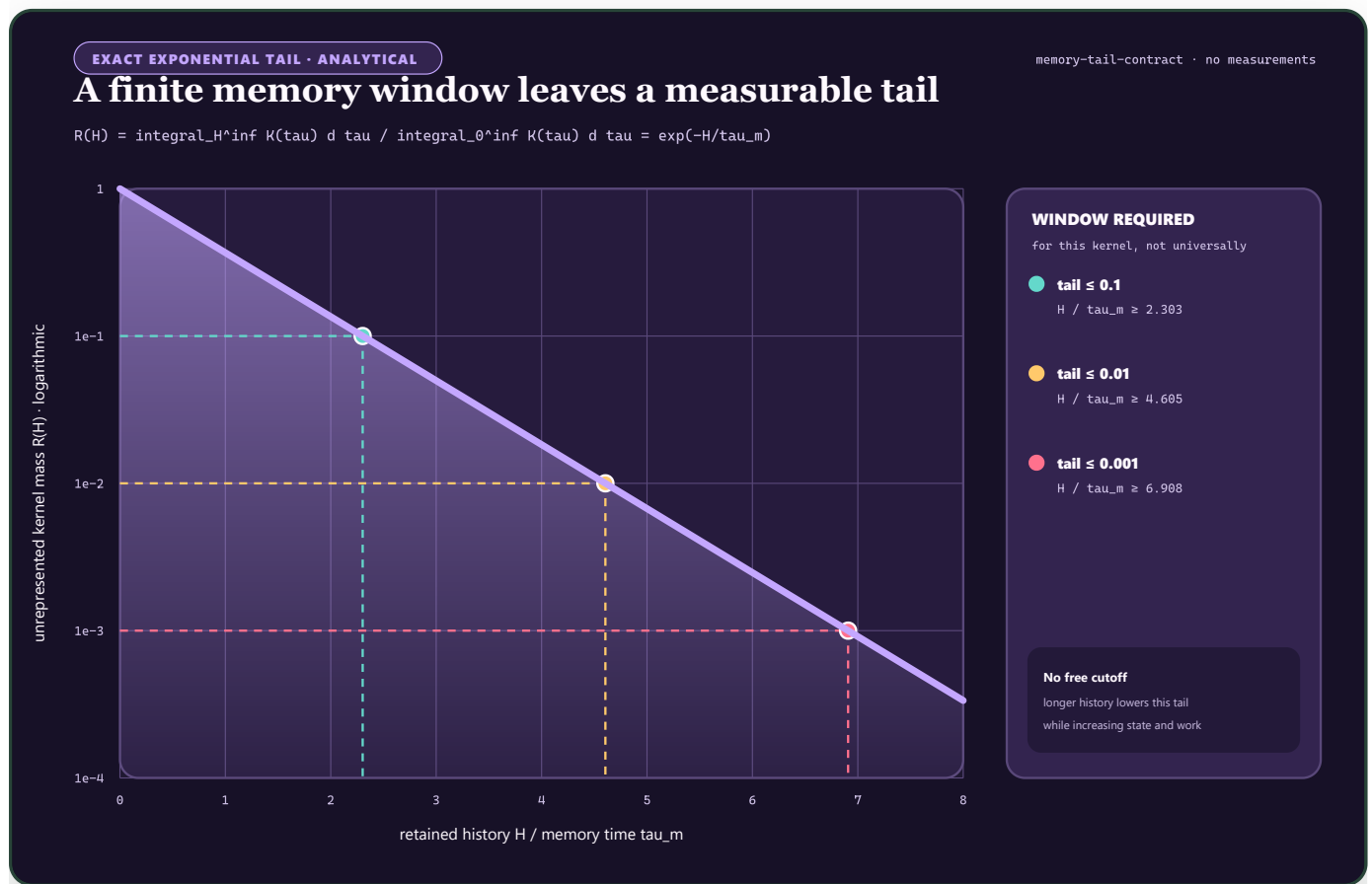
FIGURE 66 – For an exponential memory kernel, the unrepresented tail falls exponentially while every tighter tolerance requires a longer retained history.
