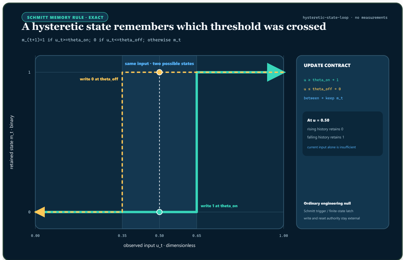
FIGURE 68 — For a binary Schmitt rule, rising and falling input histories form a loop; an input inside the threshold band is compatible with either retained state.
