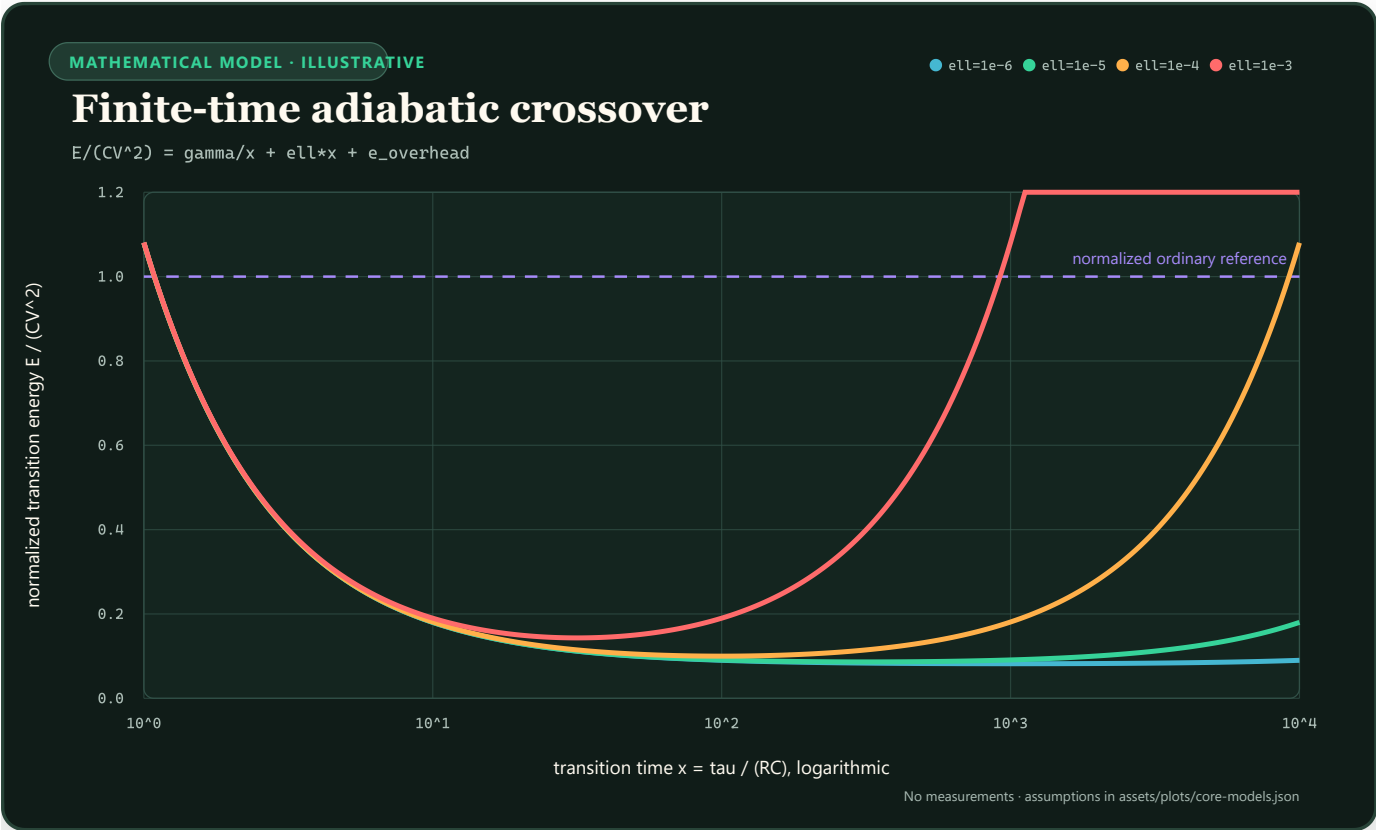
FIGURE 63 — Four normalized adiabatic energy curves form different U-shaped crossovers as leakage changes.
