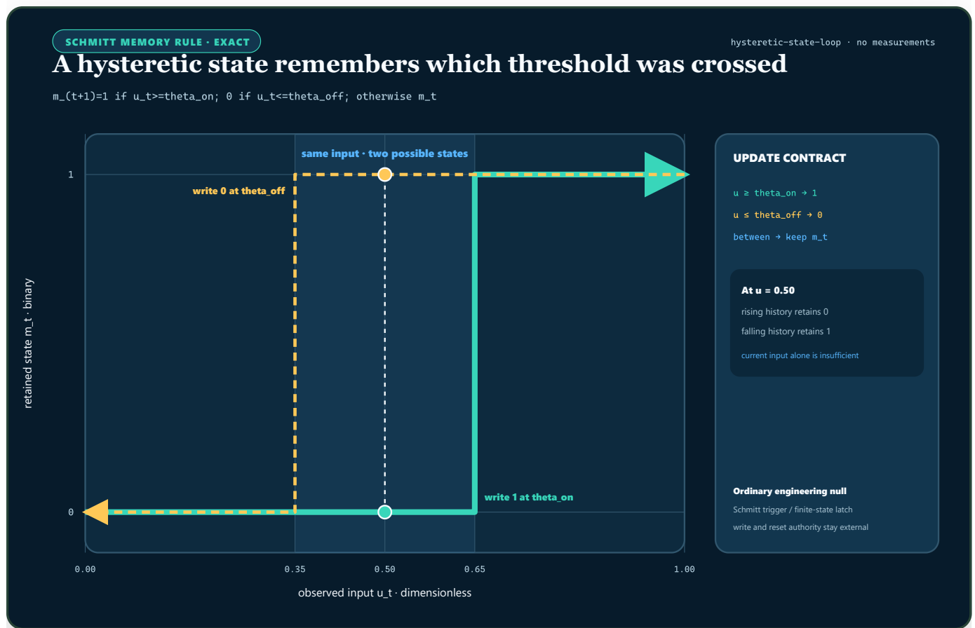
FIGURE 74 – For a binary Schmitt rule, rising and falling input histories form a loop; an input inside the threshold band is compatible with either retained state.
