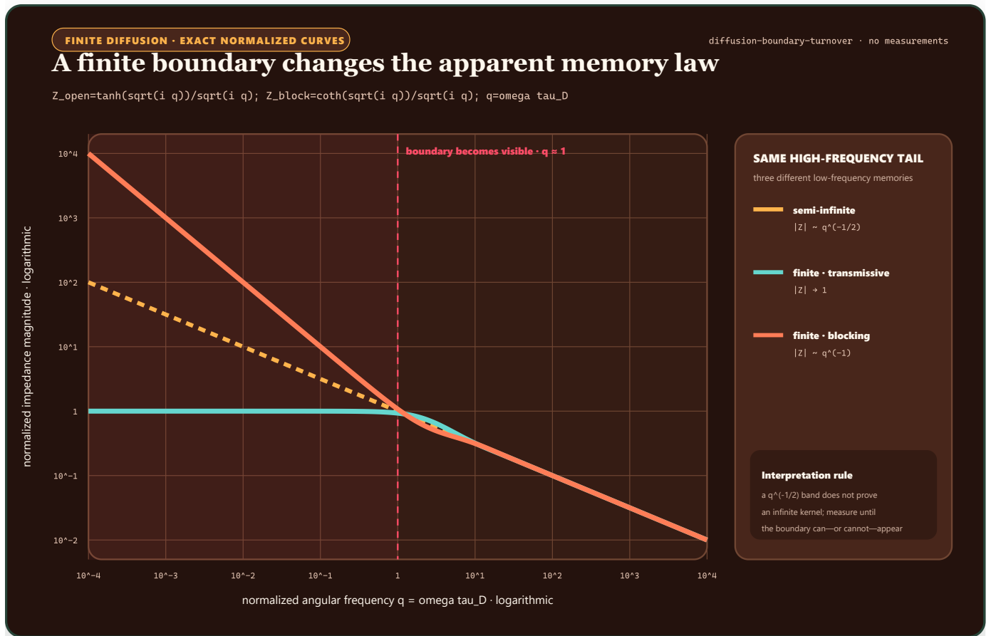
FIGURE 73 – A semi-infinite diffusion law and two finite-boundary laws coincide in their high-frequency slope but separate below the boundary timescale.
