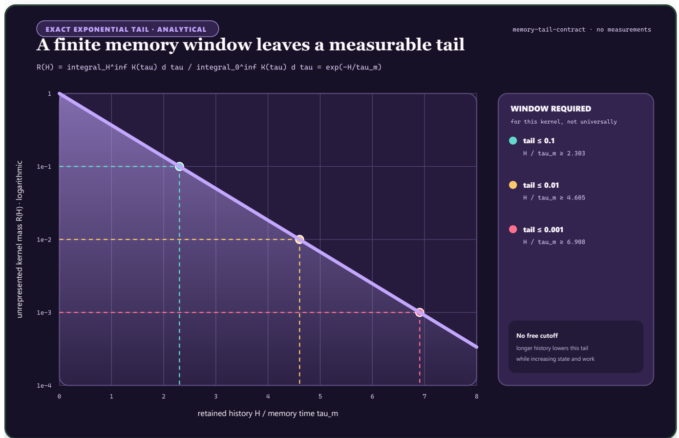
FIGURE 72 – For an exponential memory kernel, the unrepresented tail falls exponentially while every tighter tolerance requires a longer retained history.
