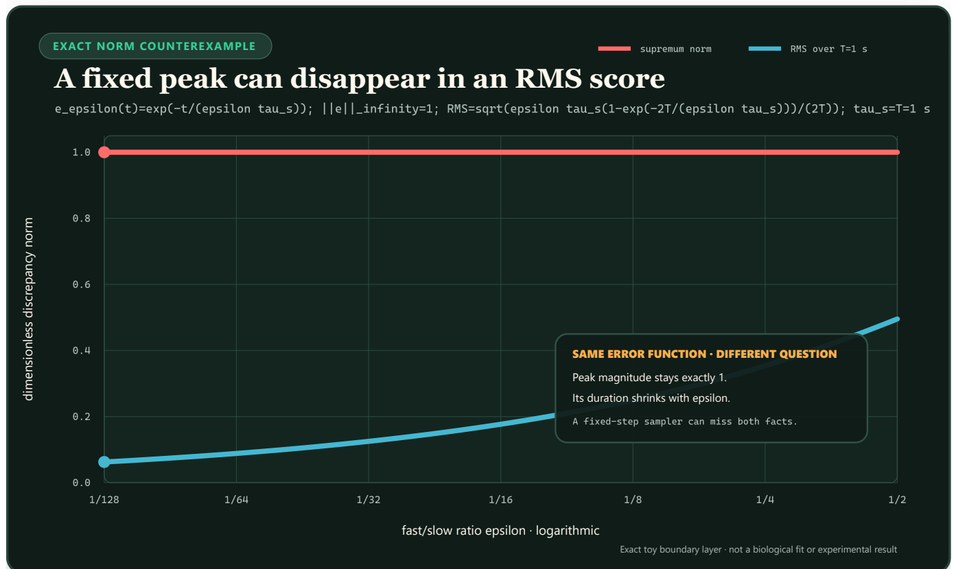
FIGURE 65 — A boundary-layer peak remains fixed in the supremum norm while its RMS value falls with epsilon.
