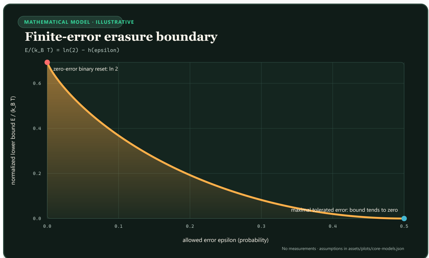
FIGURE 68 — The normalized generalized erasure lower bound falls from \ln 2 at zero error to zero at one-half allowed error.
