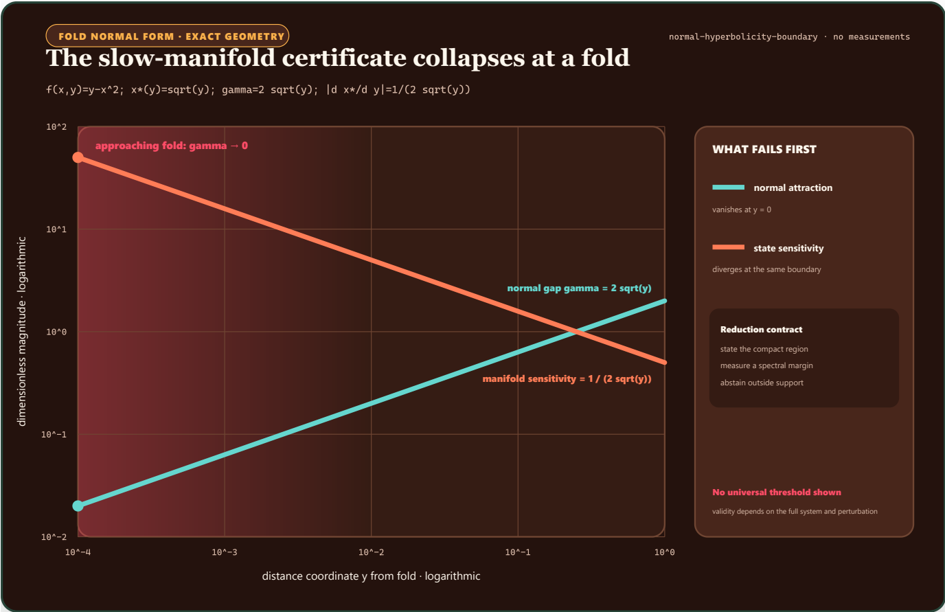
FIGURE 75 – In the fold normal form, the attracting spectral gap falls to zero while the slow-state sensitivity diverges.
