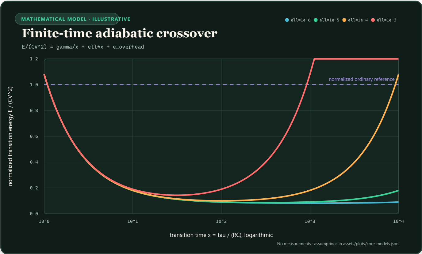
FIGURE 69 — Four normalized adiabatic energy curves form different U-shaped crossovers as leakage changes.
