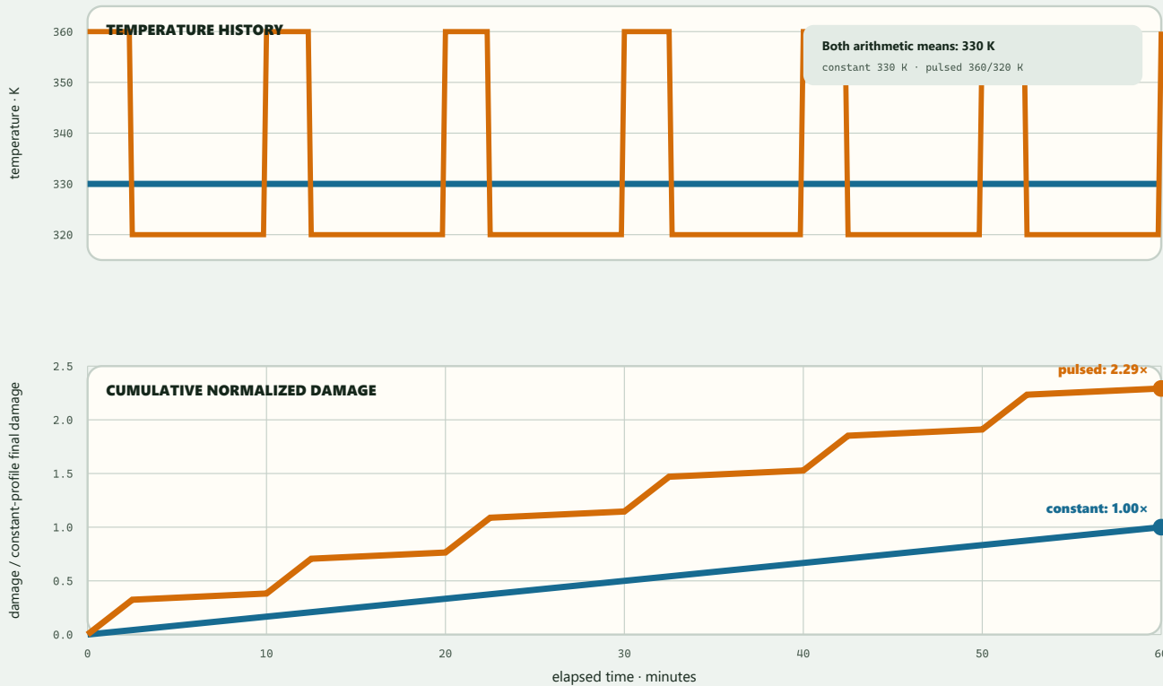
FIGURE 26 – Two devices can have the same elapsed time and arithmetic-mean temperature yet accumulate different modeled damage because the rate is nonlinear in temperature; a nominal or averaged operating point cannot replace mission history.
