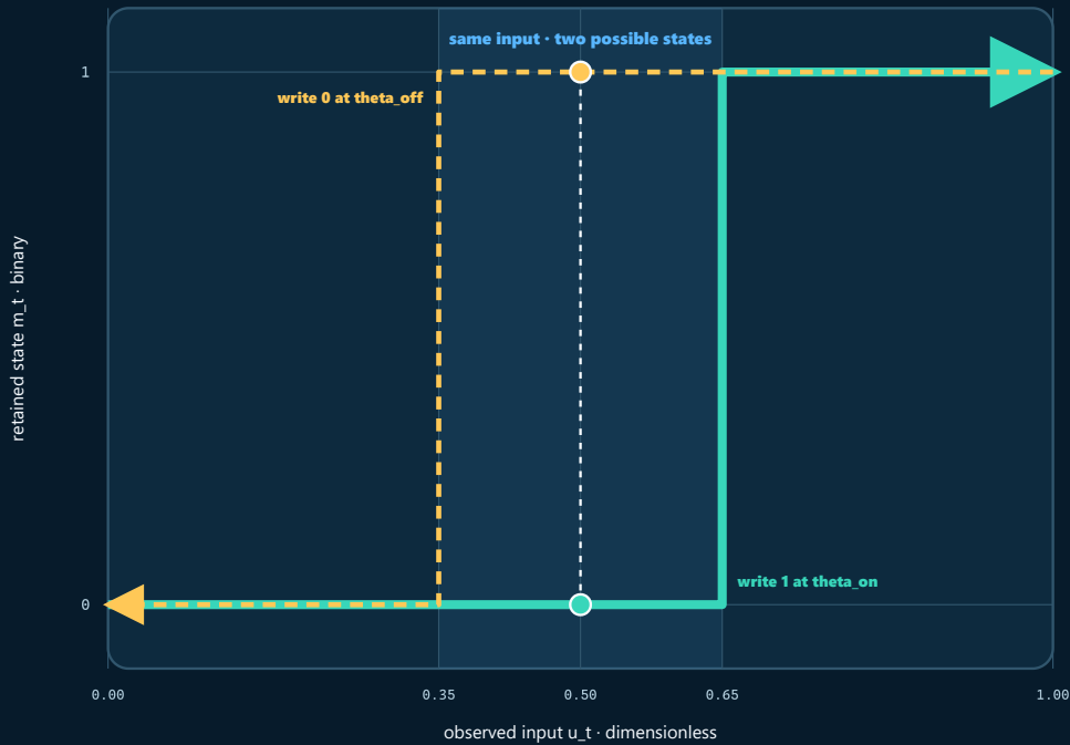
FIGURE 35 – An exact hysteresis loop for a binary Schmitt rule: inside the band, the same current input retains either zero or one according to the previously crossed threshold.
