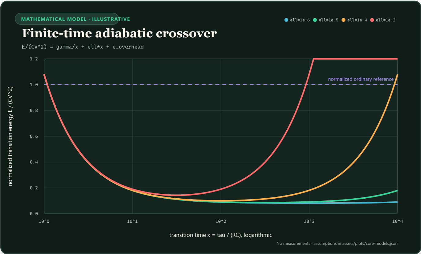
FIGURE 64 — Four normalized adiabatic energy curves form different U-shaped crossovers as leakage changes.
