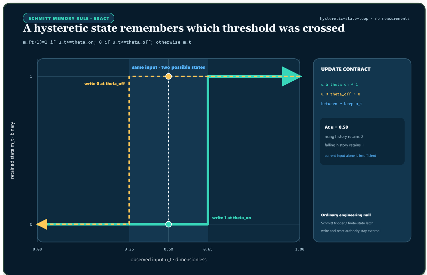
FIGURE 69 – For a binary Schmitt rule, rising and falling input histories form a loop; an input inside the threshold band is compatible with either retained state.
