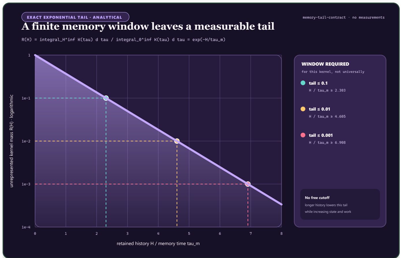
FIGURE 67 – For an exponential memory kernel, the unrepresented tail falls exponentially while every tighter tolerance requires a longer retained history.
