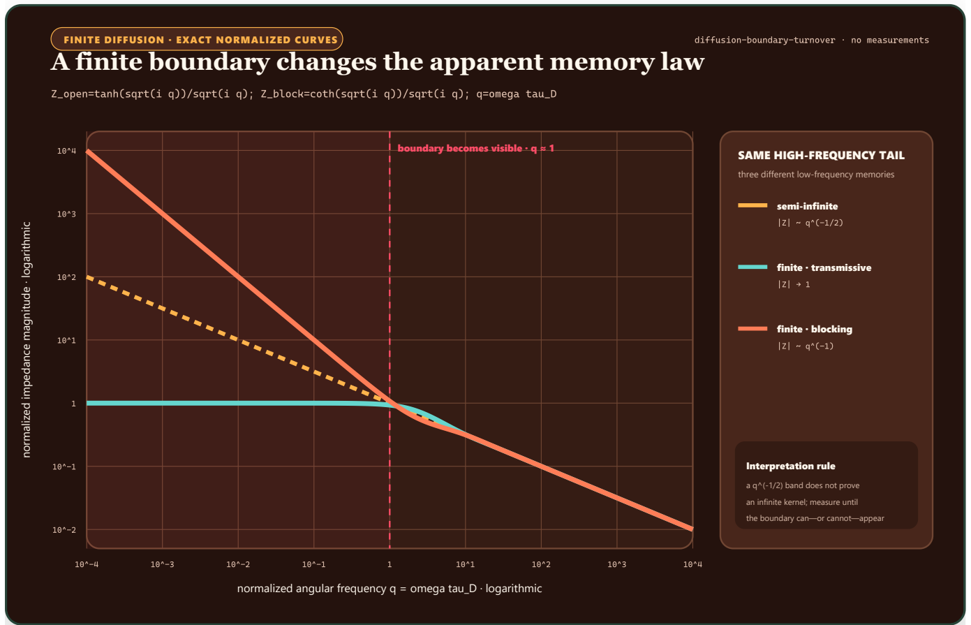
FIGURE 68 – A semi-infinite diffusion law and two finite-boundary laws coincide in their high-frequency slope but separate below the boundary timescale.
