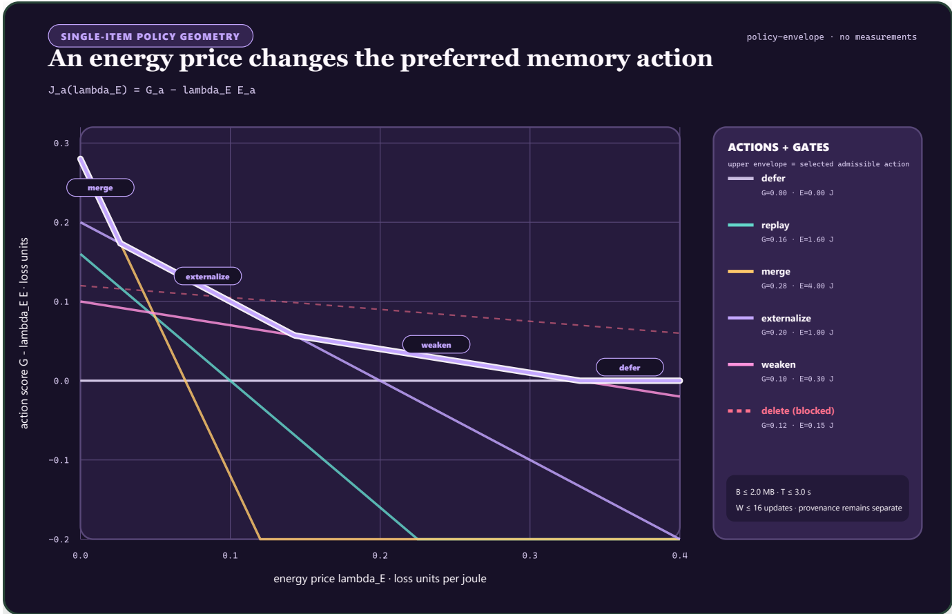
FIGURE 37 — For one memory item, each admissible action defines a score line G minus \lambda_{E_a} E ; raising the energy price can switch the selected action, while byte, time, update, provenance, and destructive-loss gates can remove an otherwise high-scoring choice.
