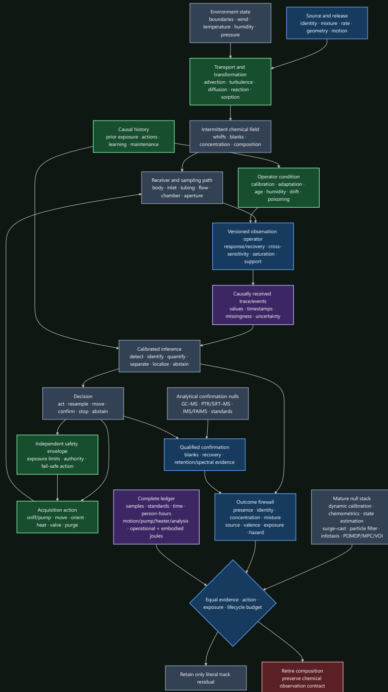
FIGURE 25 – Process diagram for One closed sensing and action contract. Key elements: Source and release · identity · mixture · rate · geometry · motion; Transport and transformation · advection · turbulence · diffusion · r....
