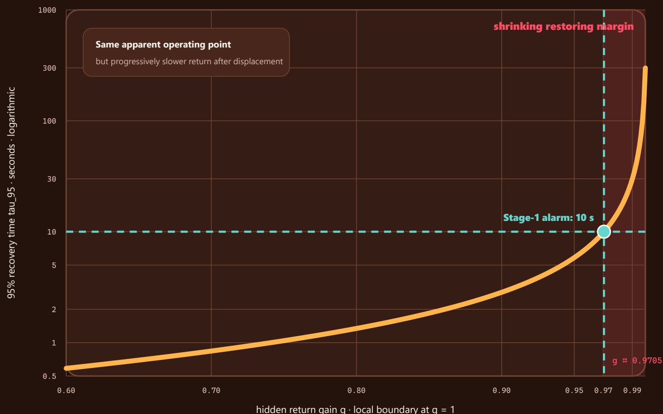
FIGURE 42 — The operating point can look unchanged while recovery time diverges as the local return gain approaches one; the ten-second line is a Stage-1 engineering threshold rather than a biological constant or predicted failure date.
