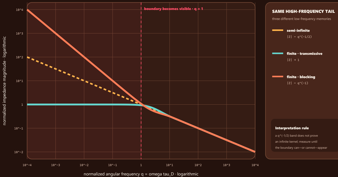
FIGURE 36 — Three normalized diffusion impedances share a high-frequency tail but split into transmissive, blocking, and semi-infinite low-frequency behavior when the boundary becomes observable.
