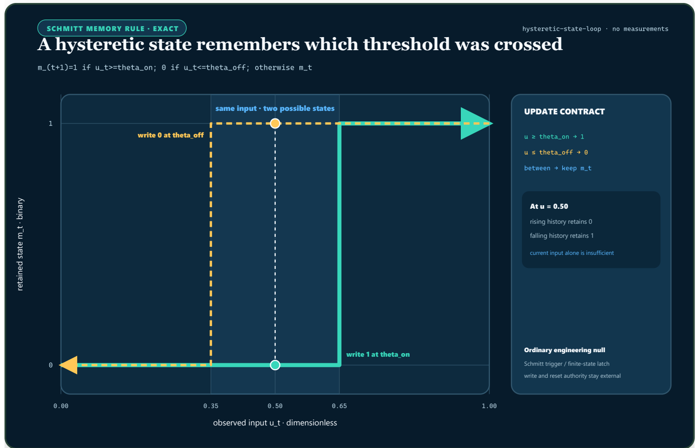
FIGURE 75 — For a binary Schmitt rule, rising and falling input histories form a loop; an input inside the threshold band is compatible with either retained state.
