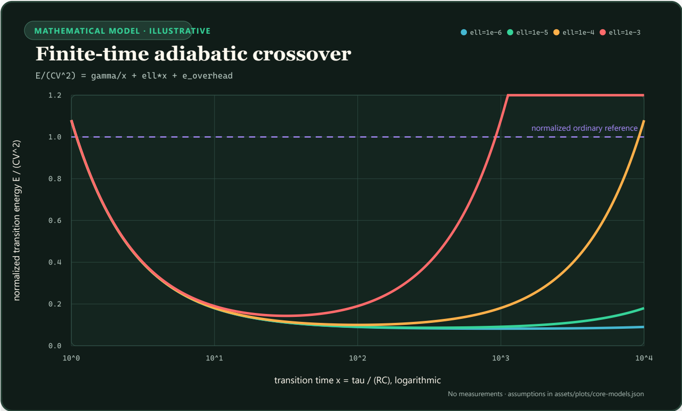
FIGURE 70 — Four normalized adiabatic energy curves form different U-shaped crossovers as leakage changes.
