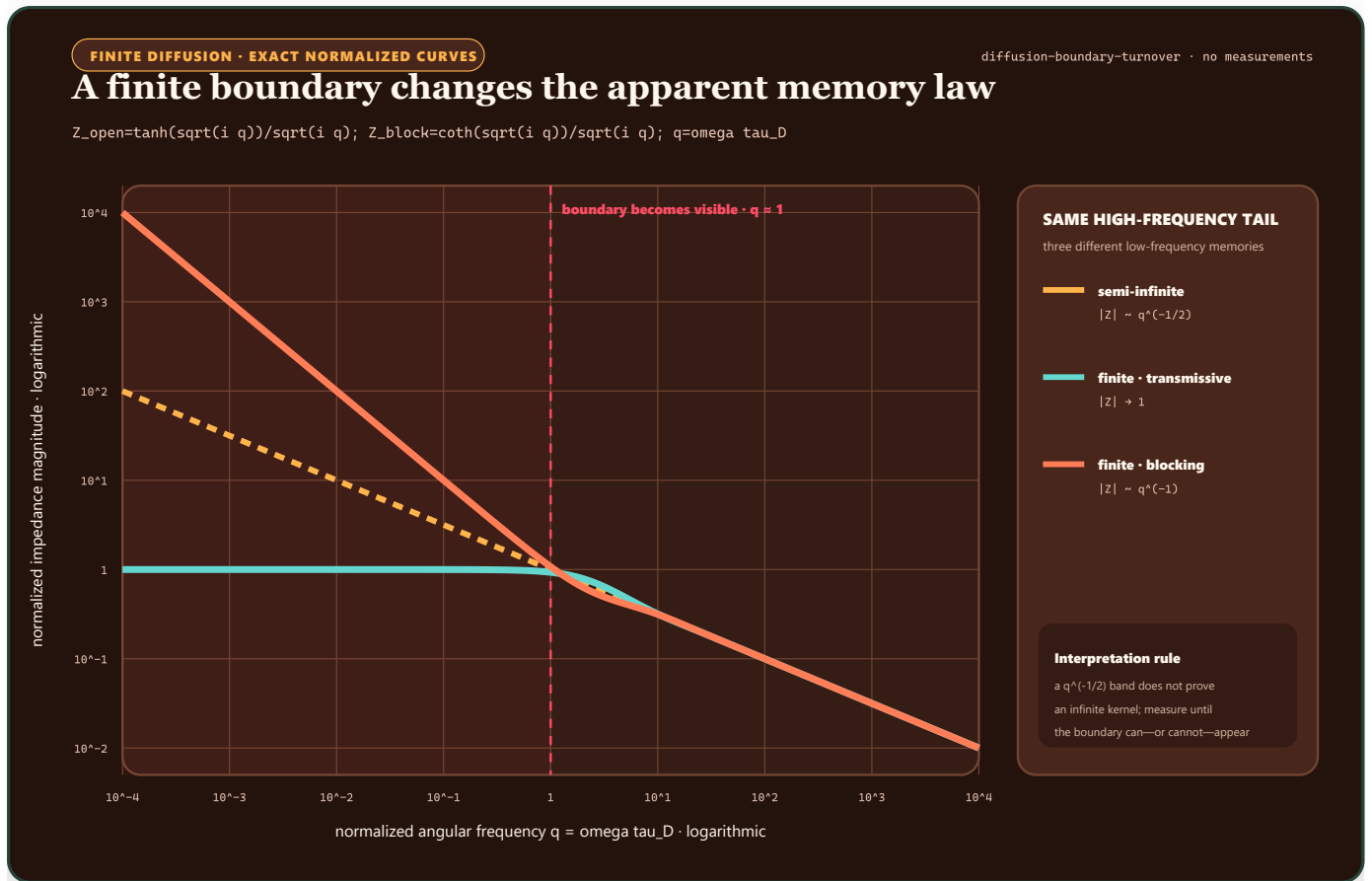
FIGURE 74 — A semi-infinite diffusion law and two finite-boundary laws coincide in their high-frequency slope but separate below the boundary timescale.
