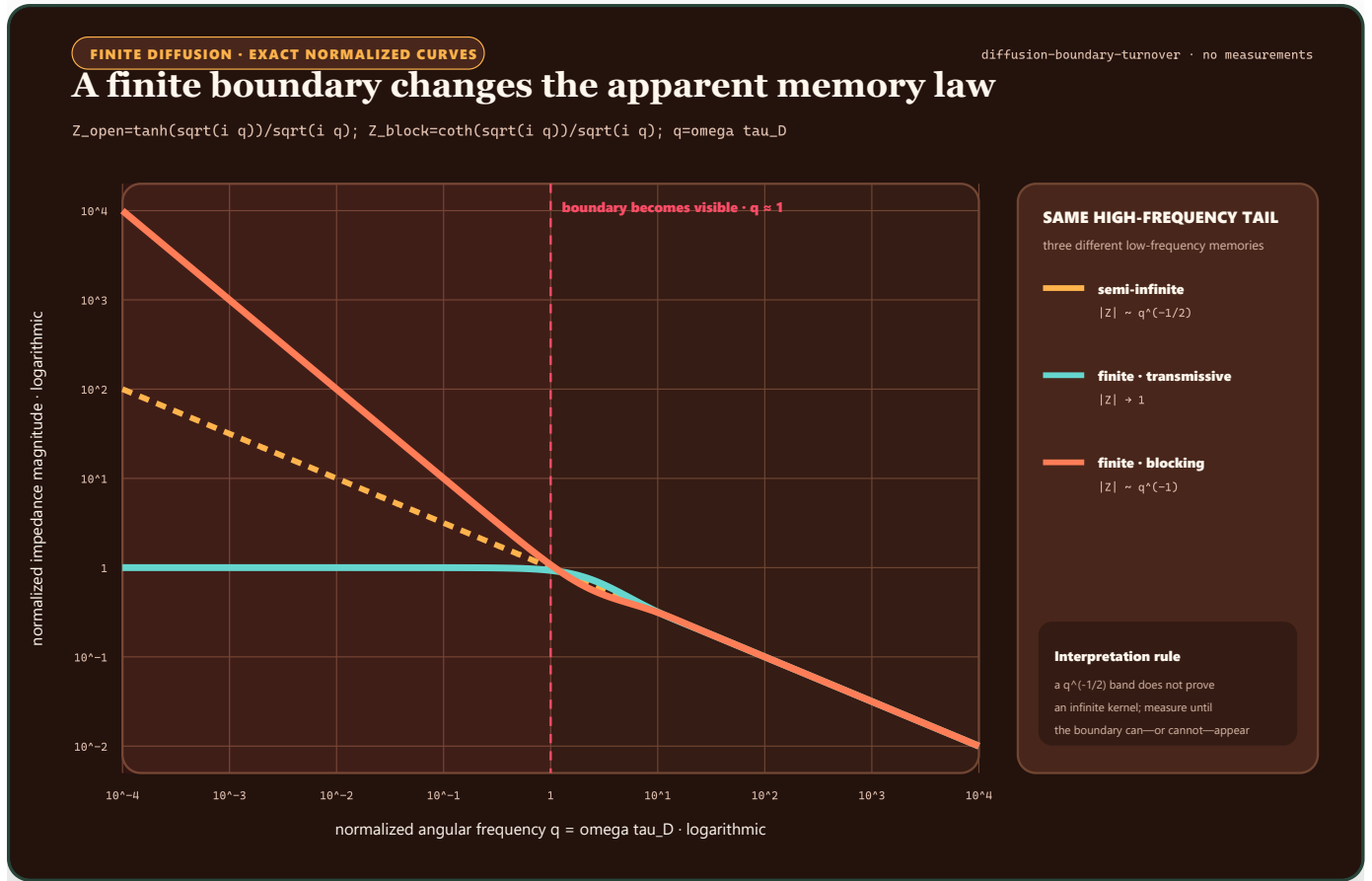
FIGURE 77 – A semi-infinite diffusion law and two finite-boundary laws coincide in their high-frequency slope but separate below the boundary timescale.
