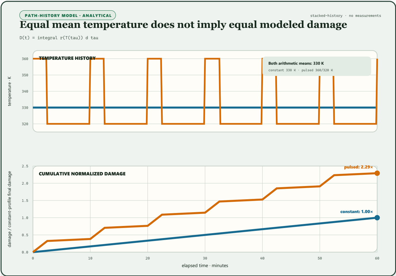
FIGURE 27 – Two devices can have the same elapsed time and arithmetic-mean temperature yet accumulate different modeled damage because the rate is nonlinear in temperature; a nominal or averaged operating point cannot replace mission history.
