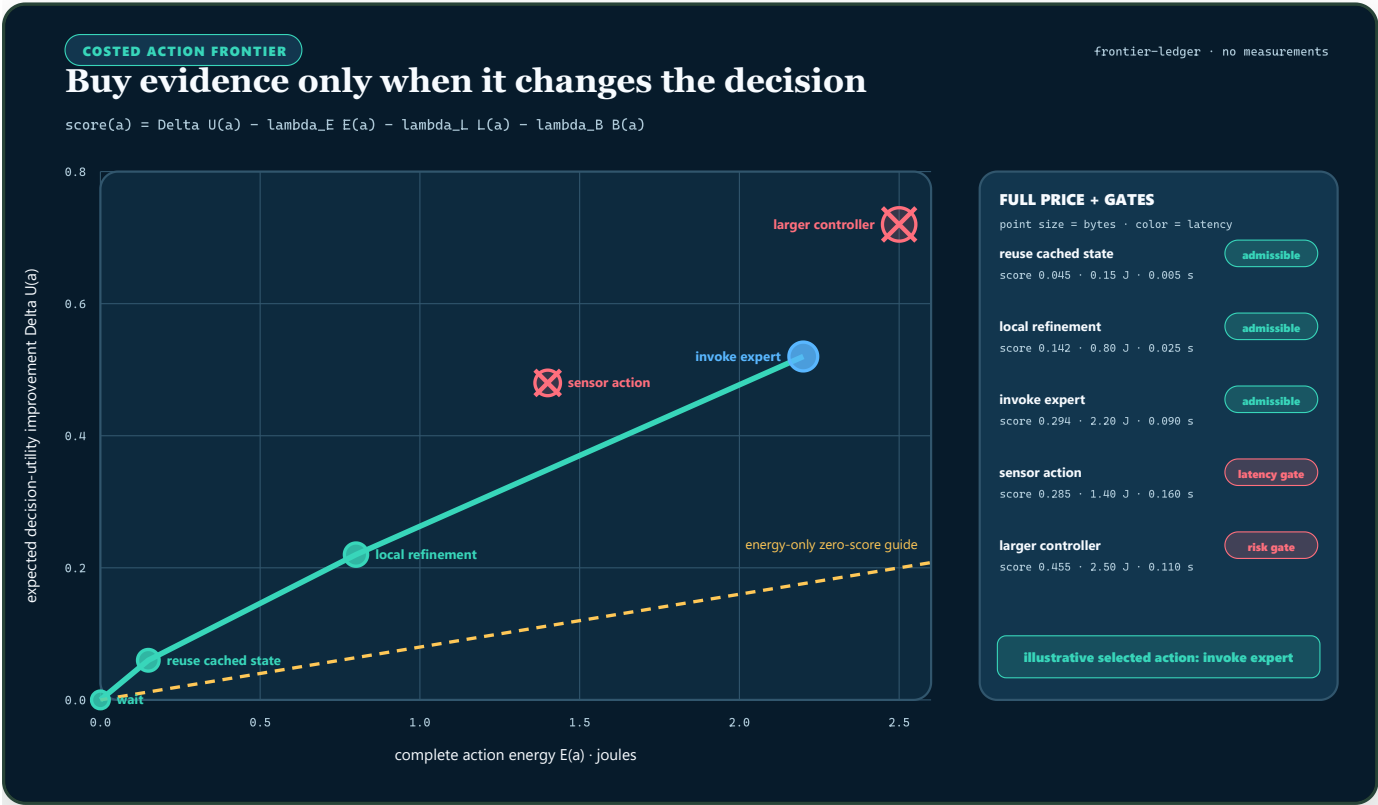
FIGURE 30 — Surprise or information gain alone does not buy another computation or measurement: an action first survives hard risk and latency gates, then competes on decision-value gain against its complete energy, delay, and traffic cost.
