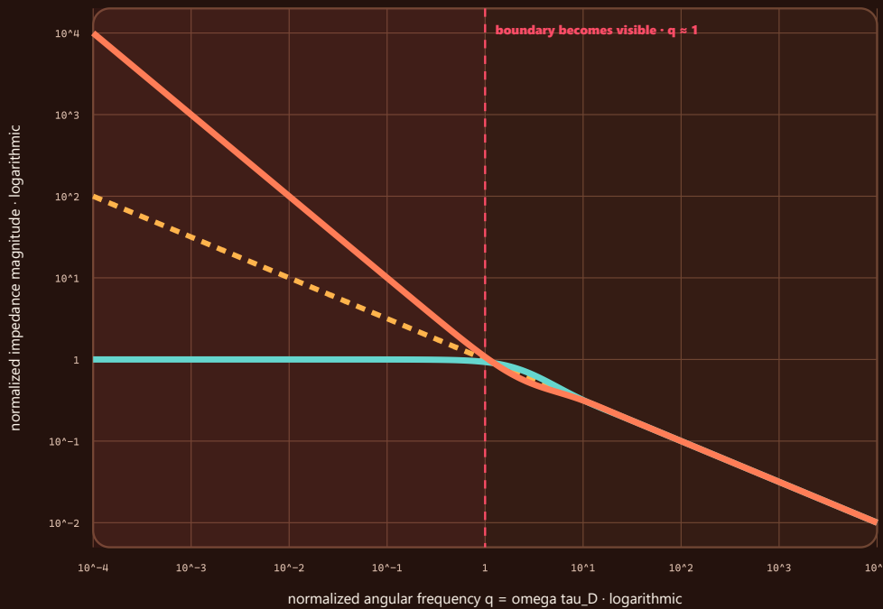
FIGURE 37 — Three normalized diffusion impedances share a high-frequency tail but split into transmissive, blocking, and semi-infinite low-frequency behavior when the boundary becomes observable.
