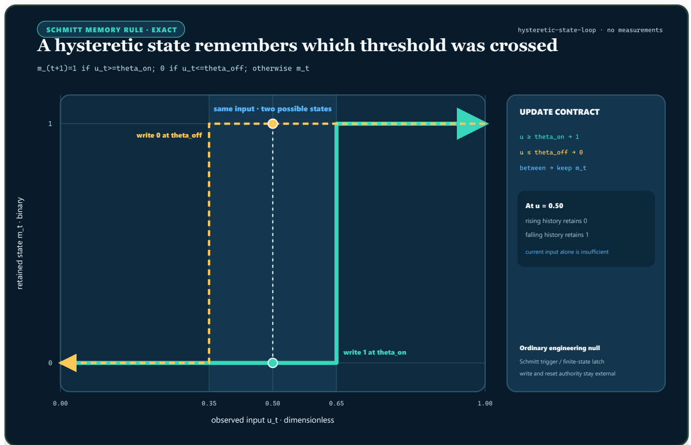
FIGURE 78 — For a binary Schmitt rule, rising and falling input histories form a loop; an input inside the threshold band is compatible with either retained state.
