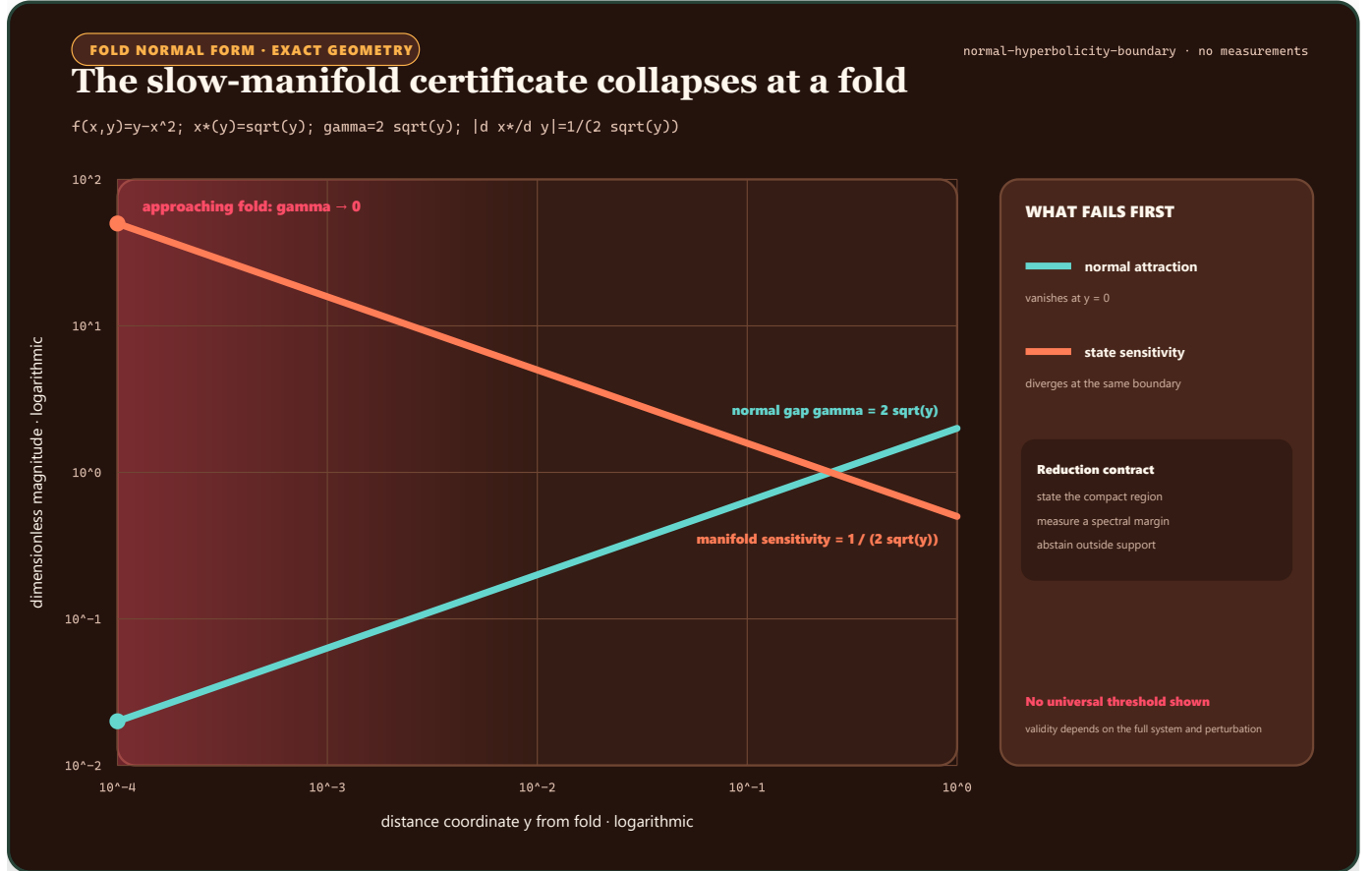
FIGURE 32 – Analytical illustration of the dimensionless fold normal form: normal attraction tends to zero and slow-branch sensitivity diverges as the dimensionless distance coordinate y approaches the fold; this is exact geometry for the displayed normal form, not a measured or universal online threshold.
