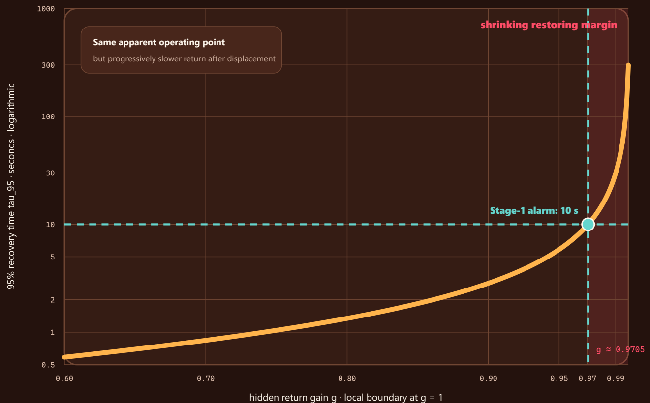
FIGURE 43 — The operating point can look unchanged while recovery time diverges as the local return gain approaches one; the ten-second line is a Stage-1 engineering threshold rather than a biological constant or predicted failure date.
