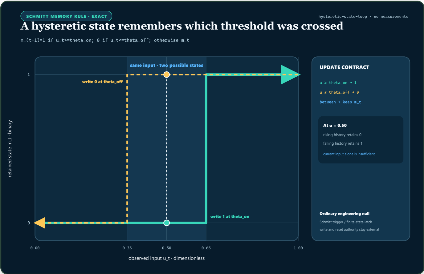
FIGURE 36 — An exact hysteresis loop for a binary Schmitt rule: inside the band, the same current input retains either zero or one according to the previously crossed threshold.
