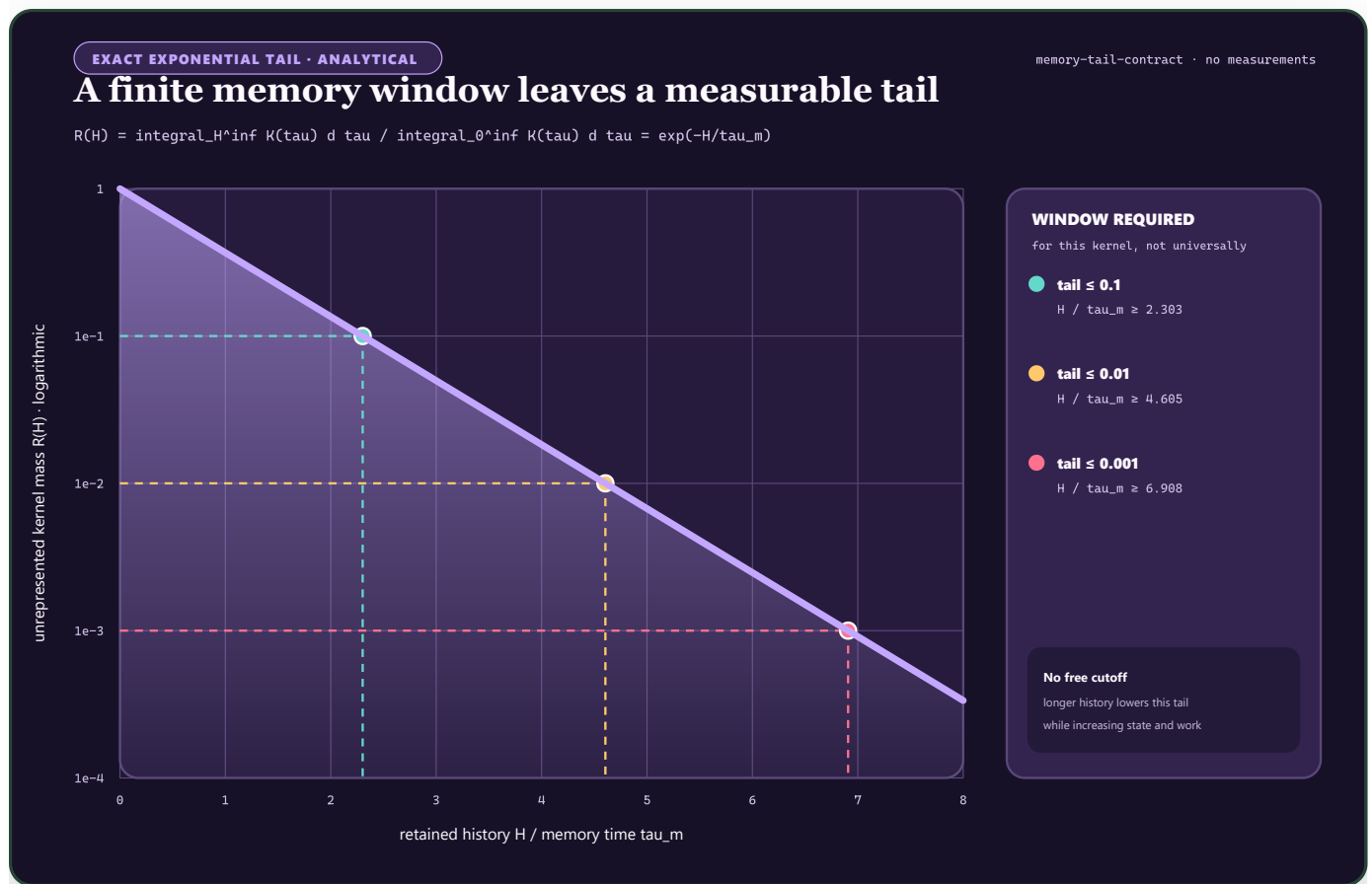
FIGURE 76 – For an exponential memory kernel, the unrepresented tail falls exponentially while every tighter tolerance requires a longer retained history.
