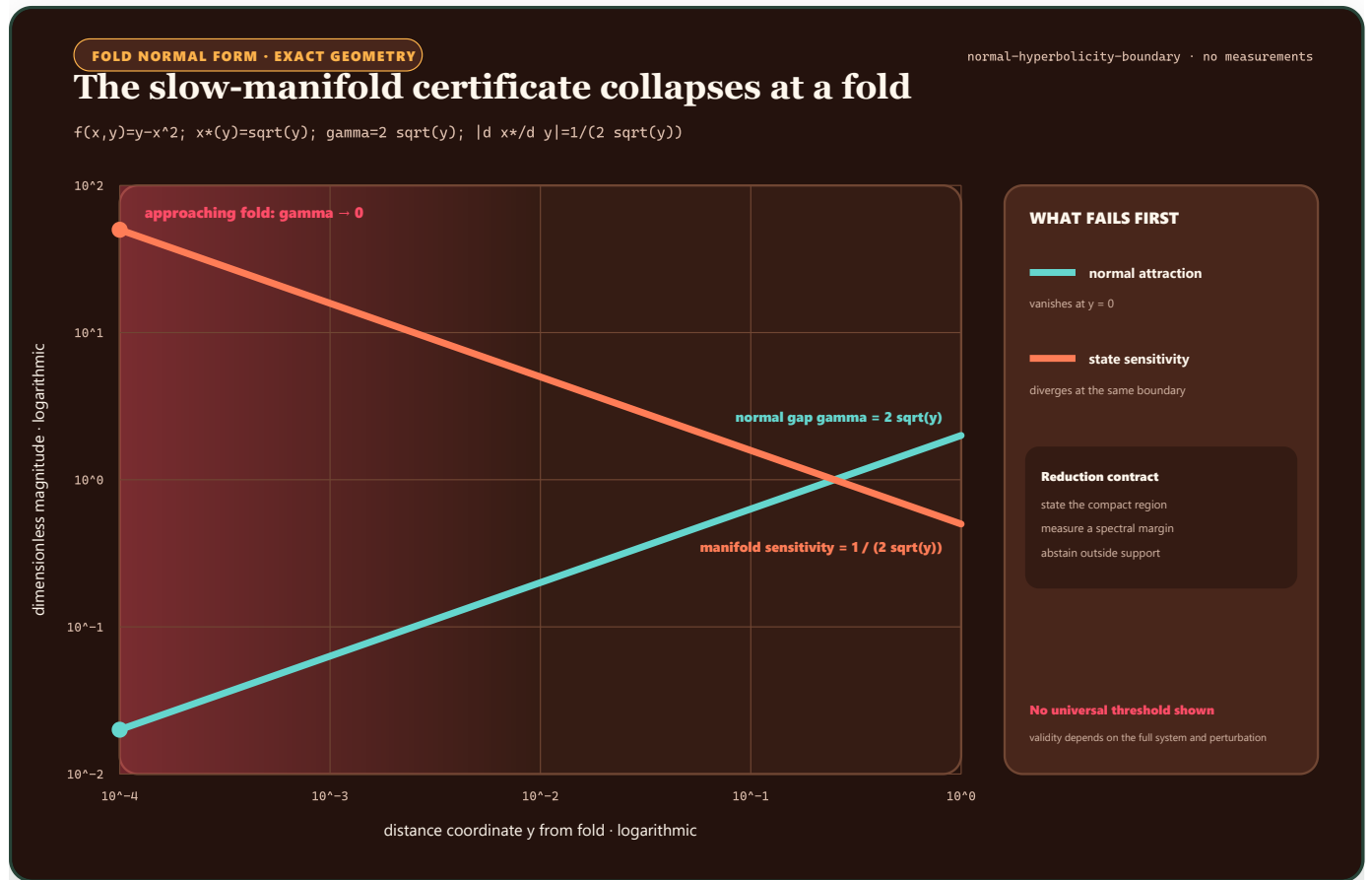
FIGURE 79 – In the fold normal form, the attracting spectral gap falls to zero while the slow-state sensitivity diverges.
