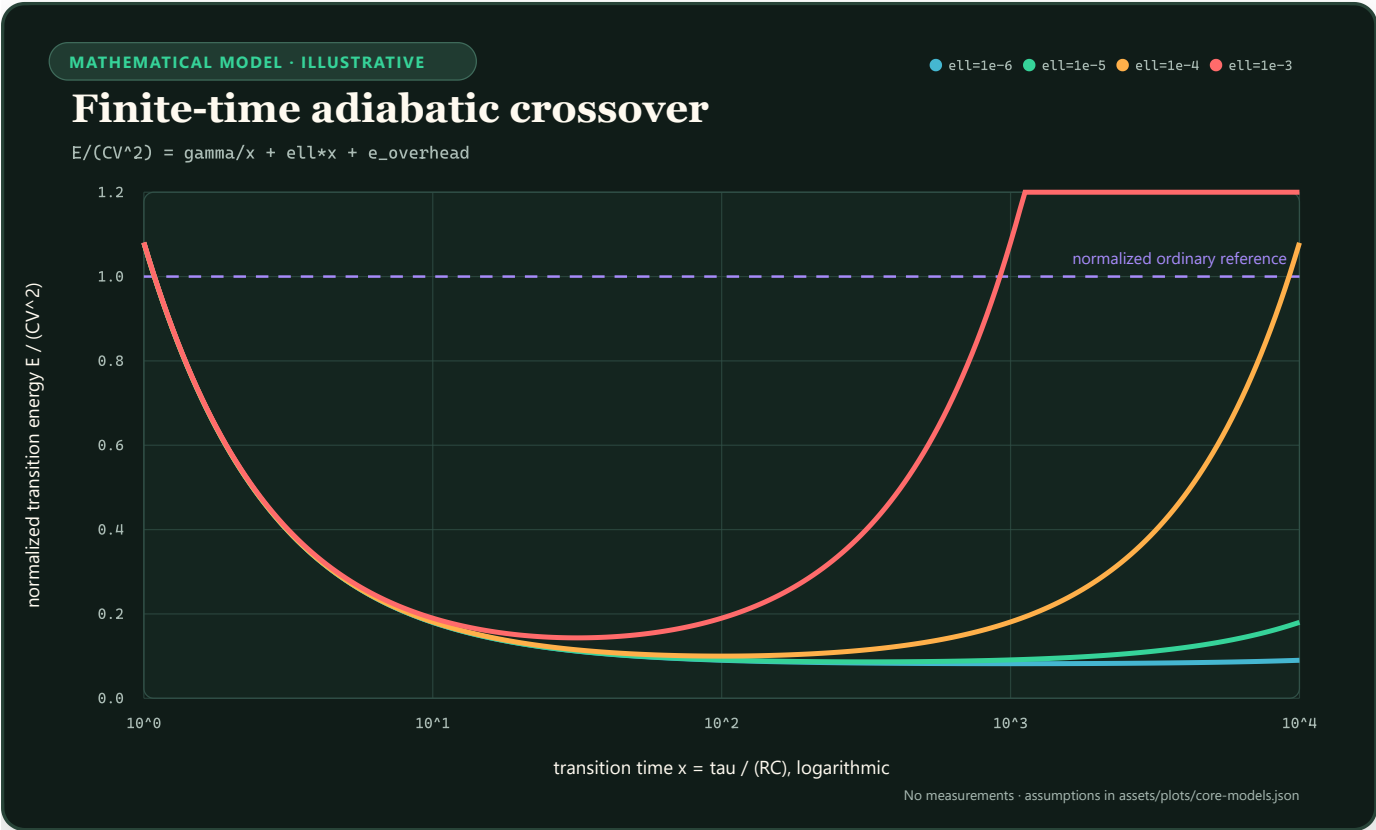
FIGURE 73 — Four normalized adiabatic energy curves form different U-shaped crossovers as leakage changes.
