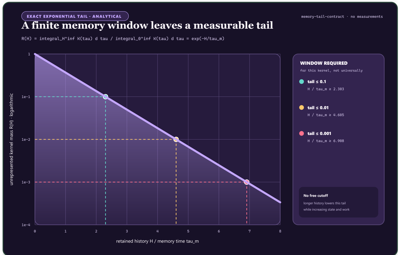
FIGURE 31 – Analytical illustration of the exact normalized tail left by truncating one exponential memory kernel; the horizontal coordinate H divided by \tau_m and the tail mass are dimensionless, and no workload measurements are shown.
