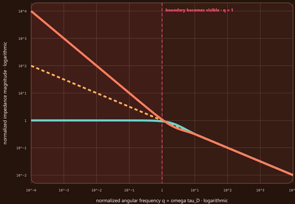
FIGURE 36 — Three normalized diffusion impedances share a high-frequency tail but split into transmissive, blocking, and semi-infinite low-frequency behavior when the boundary becomes observable.
