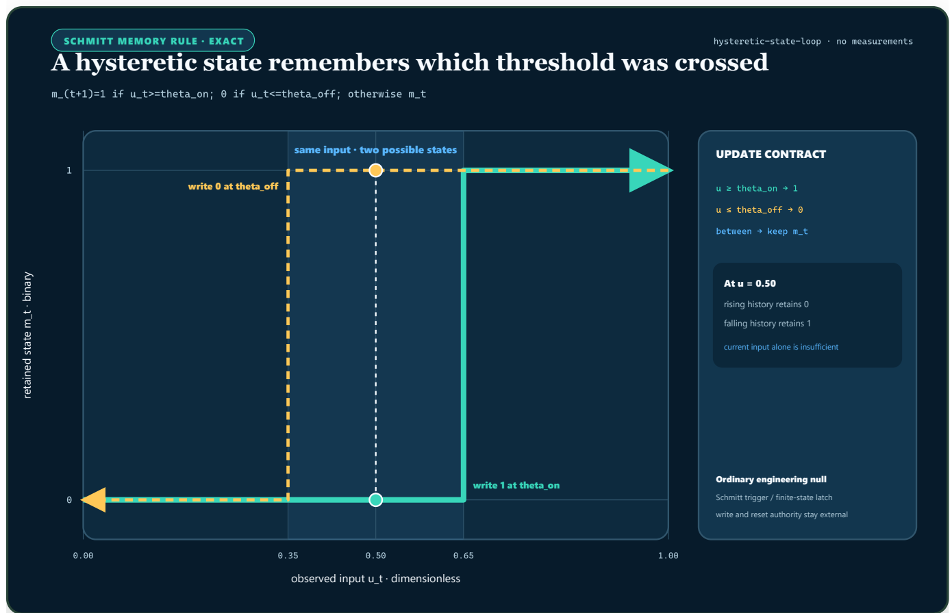
FIGURE 71 — For a binary Schmitt rule, rising and falling input histories form a loop; an input inside the threshold band is compatible with either retained state.
