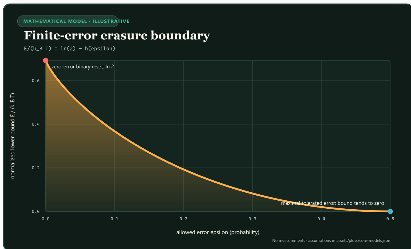
FIGURE 65 — The normalized generalized erasure lower bound falls from \ln 2 at zero error to zero at one-half allowed error.
