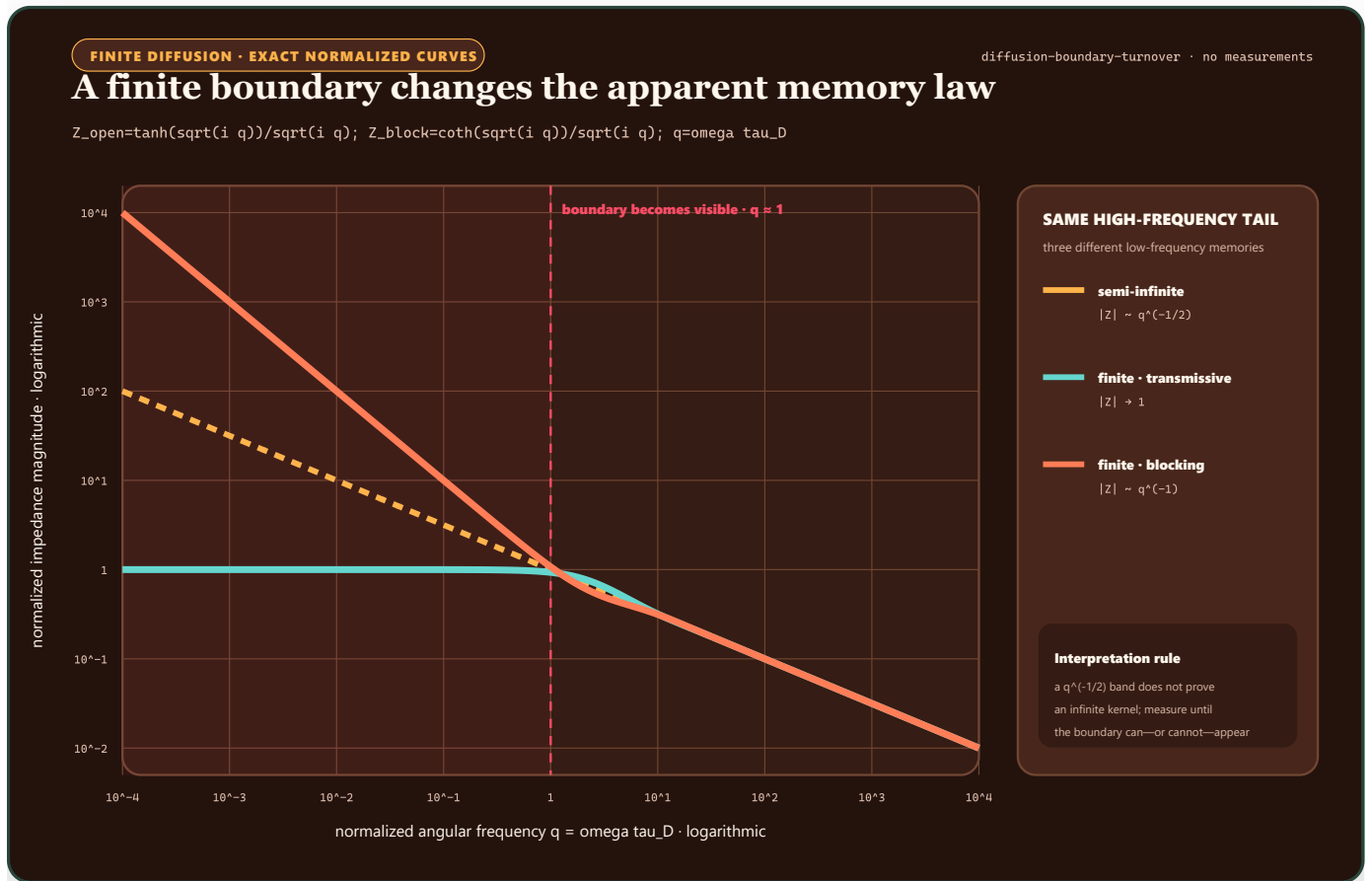
FIGURE 70 — A semi-infinite diffusion law and two finite-boundary laws coincide in their high-frequency slope but separate below the boundary timescale.
