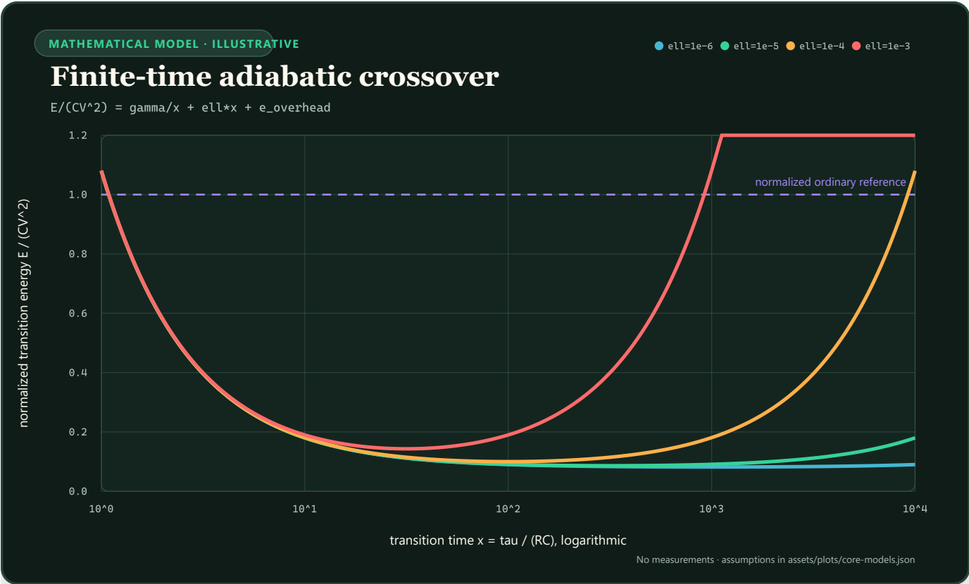
FIGURE 66 — Four normalized adiabatic energy curves form different U-shaped crossovers as leakage changes.
