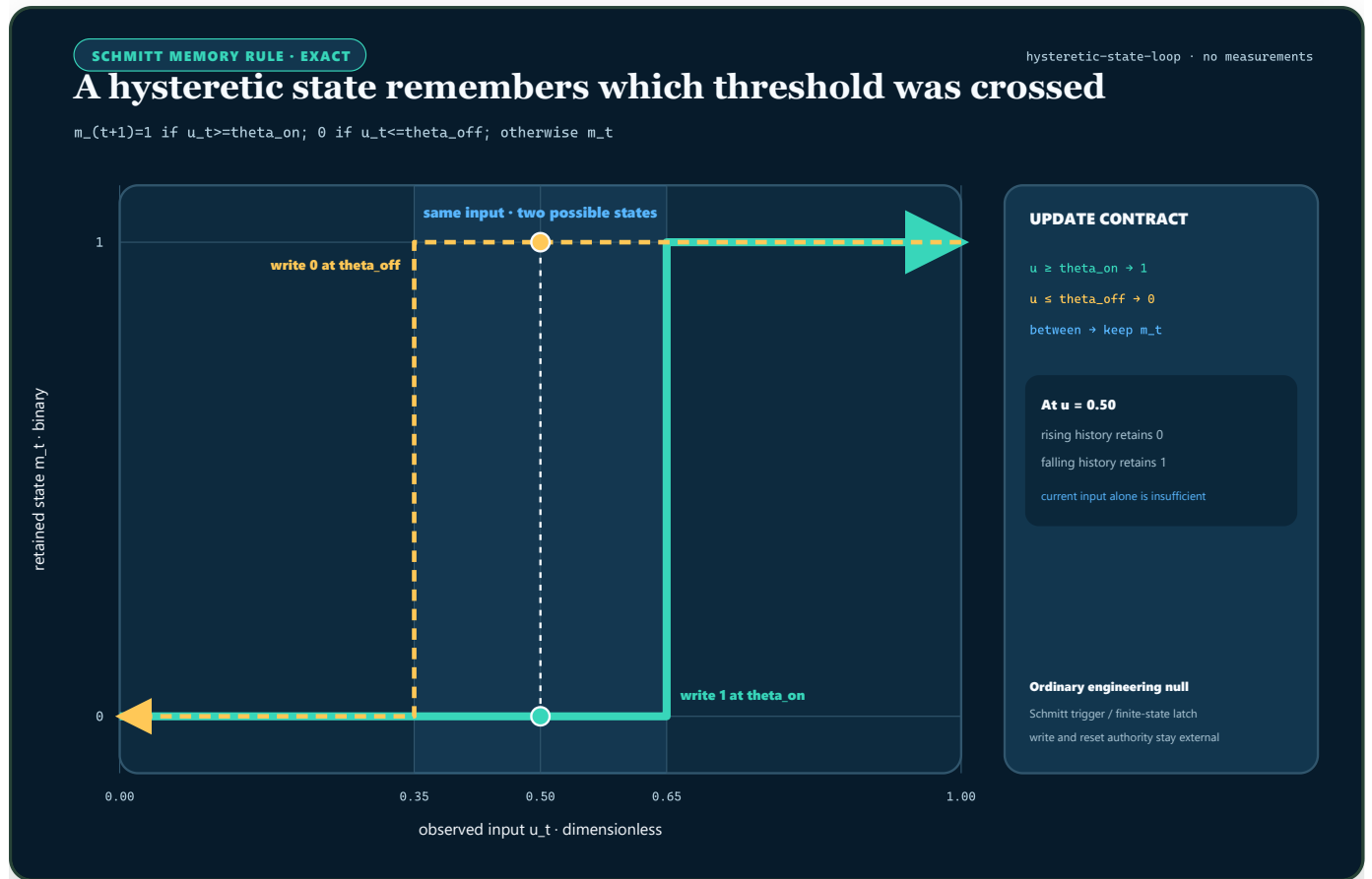
FIGURE 66 — For a binary Schmitt rule, rising and falling input histories form a loop; an input inside the threshold band is compatible with either retained state.
