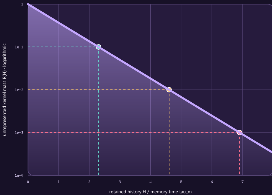
FIGURE 30 – Analytical illustration of the exact normalized tail left by truncating one exponential memory kernel; the horizontal coordinate H divided by \tau_m and the tail mass are dimensionless, and no workload measurements are shown.
