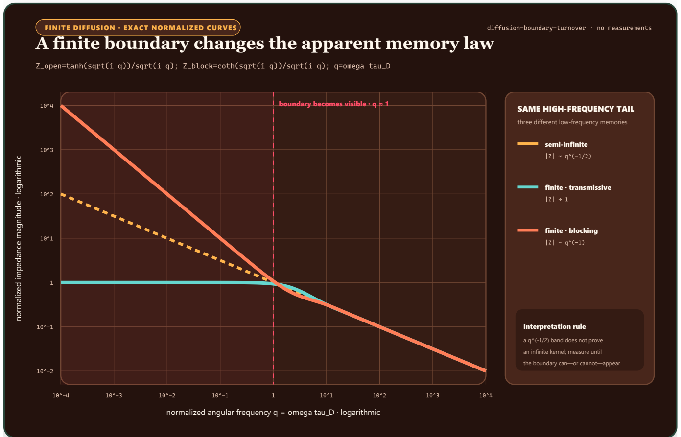
FIGURE 65 – A semi-infinite diffusion law and two finite-boundary laws coincide in their high-frequency slope but separate below the boundary timescale.
