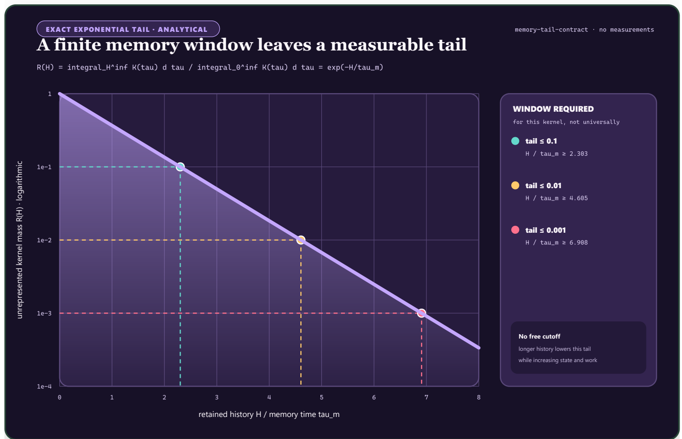
FIGURE 64 — For an exponential memory kernel, the unrepresented tail falls exponentially while every tighter tolerance requires a longer retained history.
