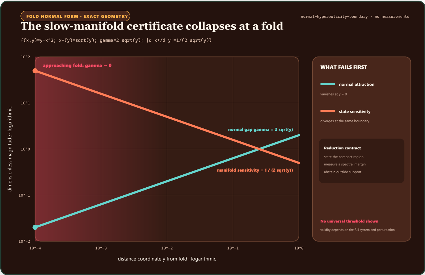
FIGURE 73 – In the fold normal form, the attracting spectral gap falls to zero while the slow-state sensitivity diverges.
