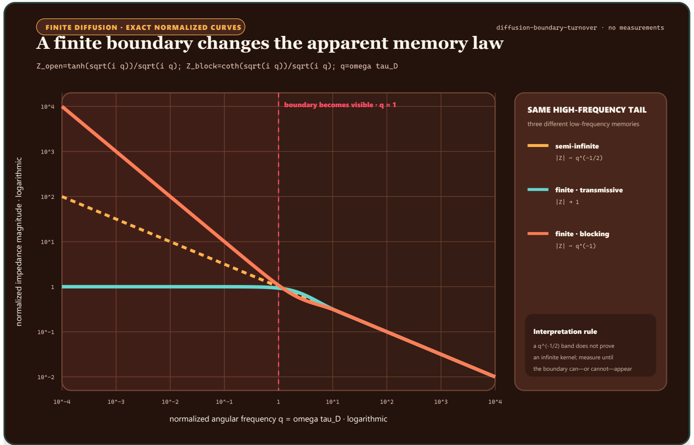
FIGURE 71 – A semi-infinite diffusion law and two finite-boundary laws coincide in their high-frequency slope but separate below the boundary timescale.
