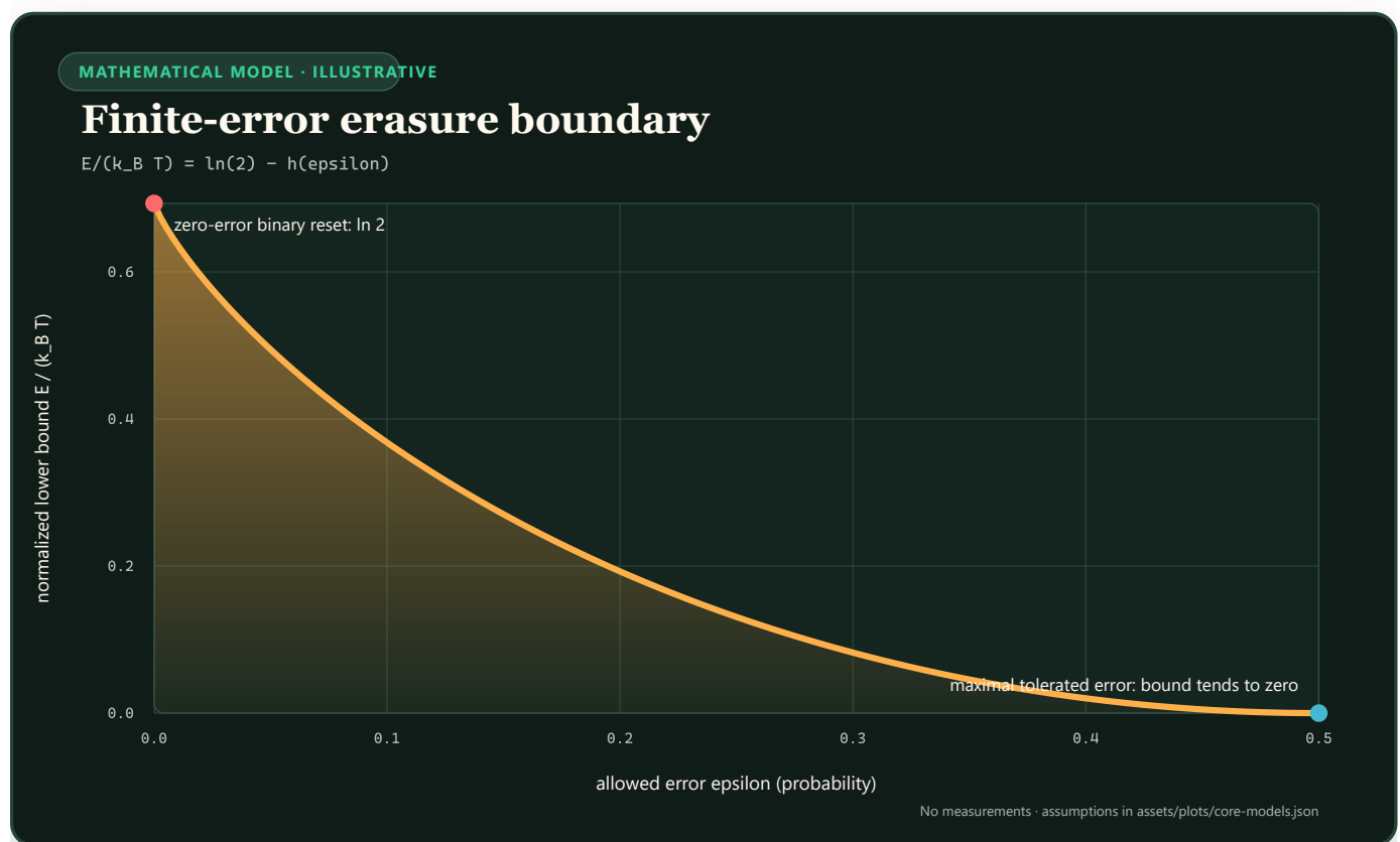
FIGURE 66 — The normalized generalized erasure lower bound falls from \ln 2 at zero error to zero at one-half allowed error.
