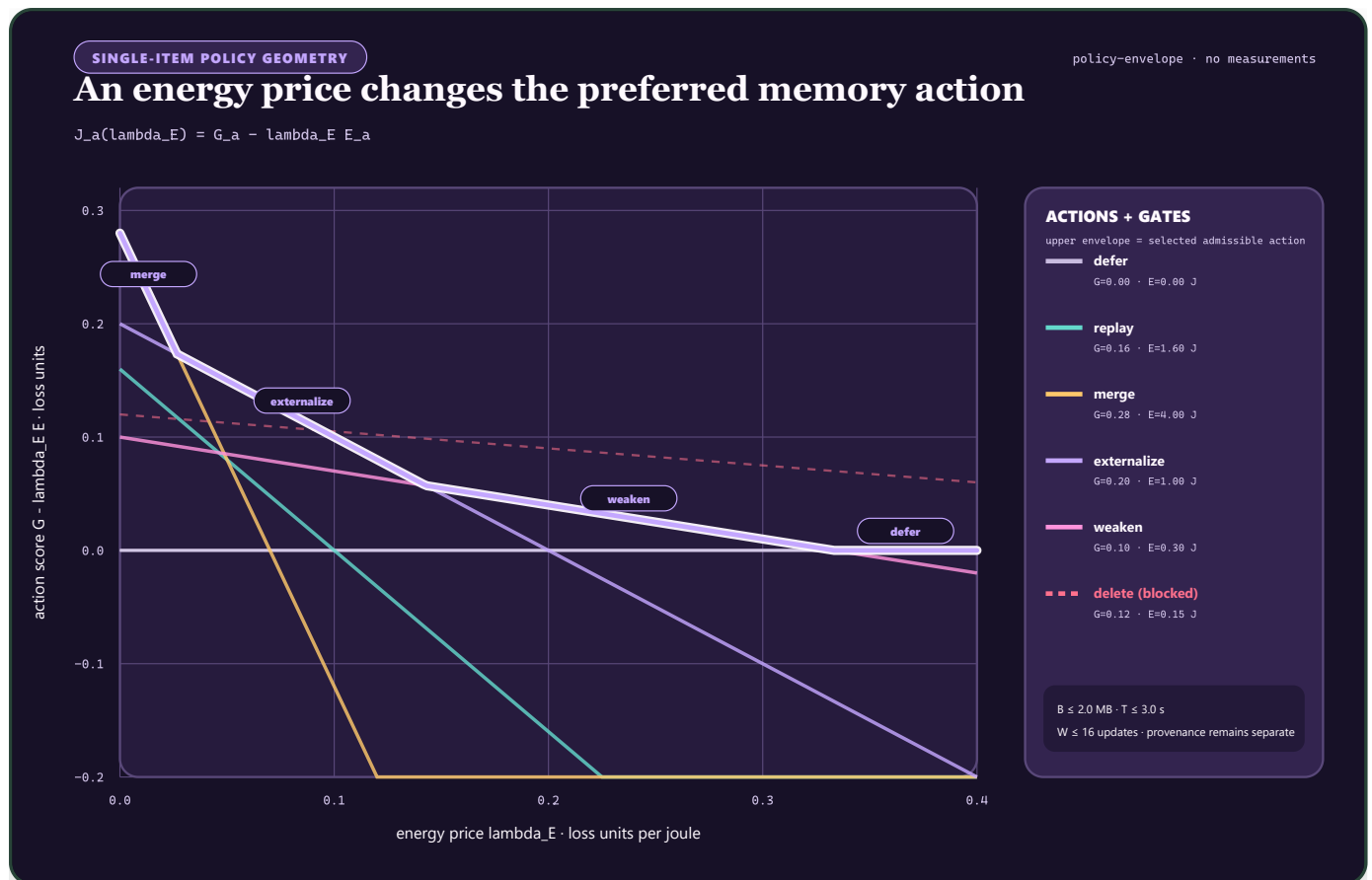
FIGURE 38 — For one memory item, each admissible action defines a score line G minus \lambda_{E_a} E ; raising the energy price can switch the selected action, while byte, time, update, provenance, and destructive-loss gates can remove an otherwise high-scoring choice.
