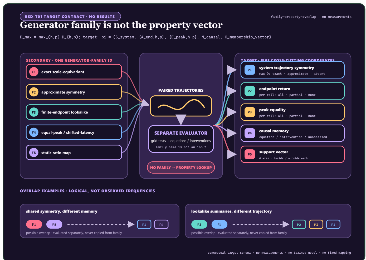
FIGURE 63 — Five generator-family labels converge through paired trajectories into a separate evaluator, which produces five cross-cutting property coordinates while retaining logical dependencies; two examples show that different families can share properties while differing on others.
