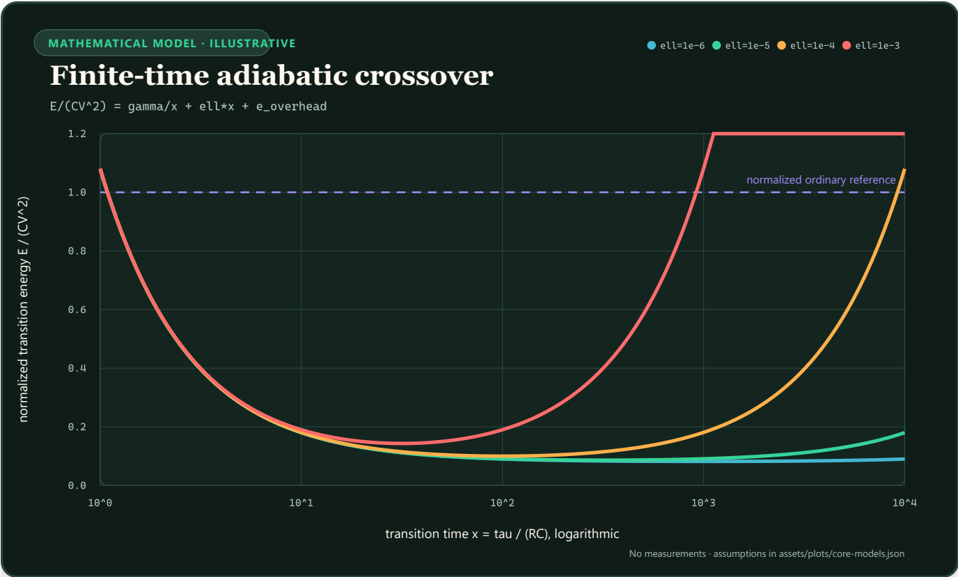
FIGURE 57 — Four normalized adiabatic energy curves form different U-shaped crossovers as leakage changes.
