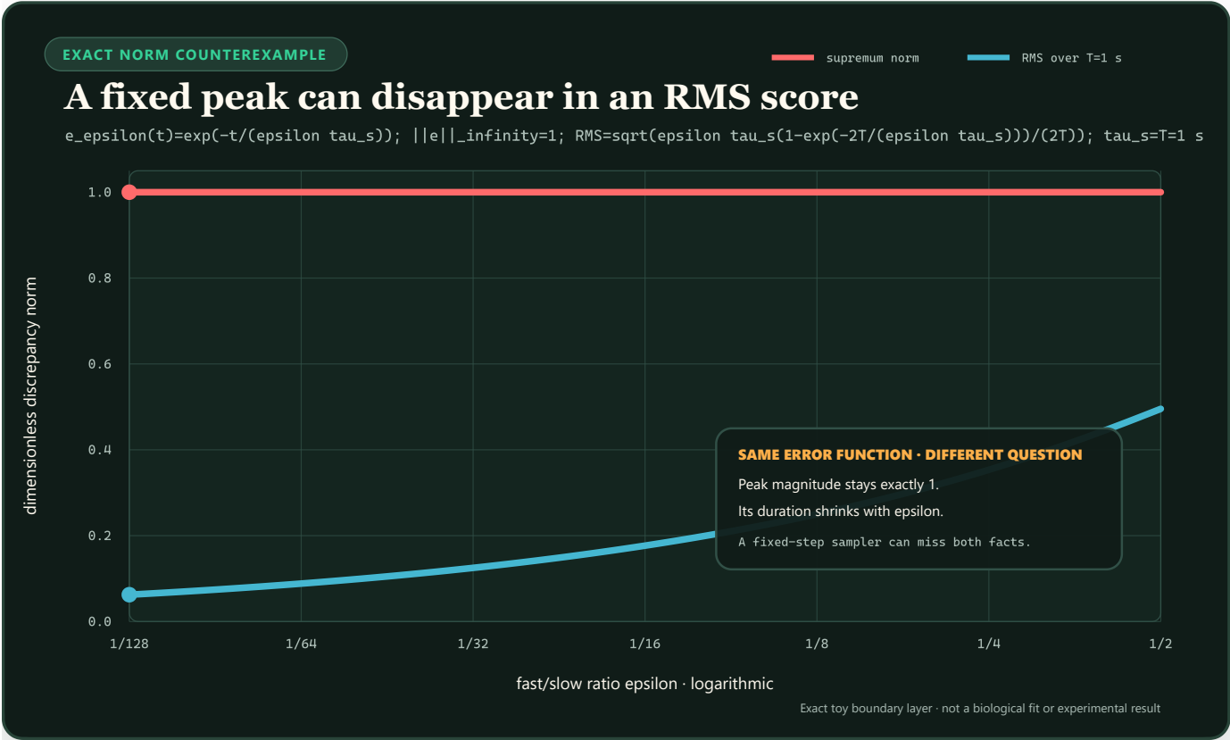
FIGURE 64 — A boundary-layer peak remains fixed in the supremum norm while its RMS value falls with epsilon.
