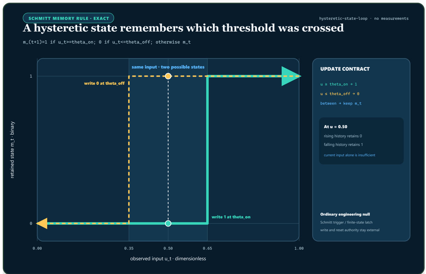
FIGURE 73 – For a binary Schmitt rule, rising and falling input histories form a loop; an input inside the threshold band is compatible with either retained state.
