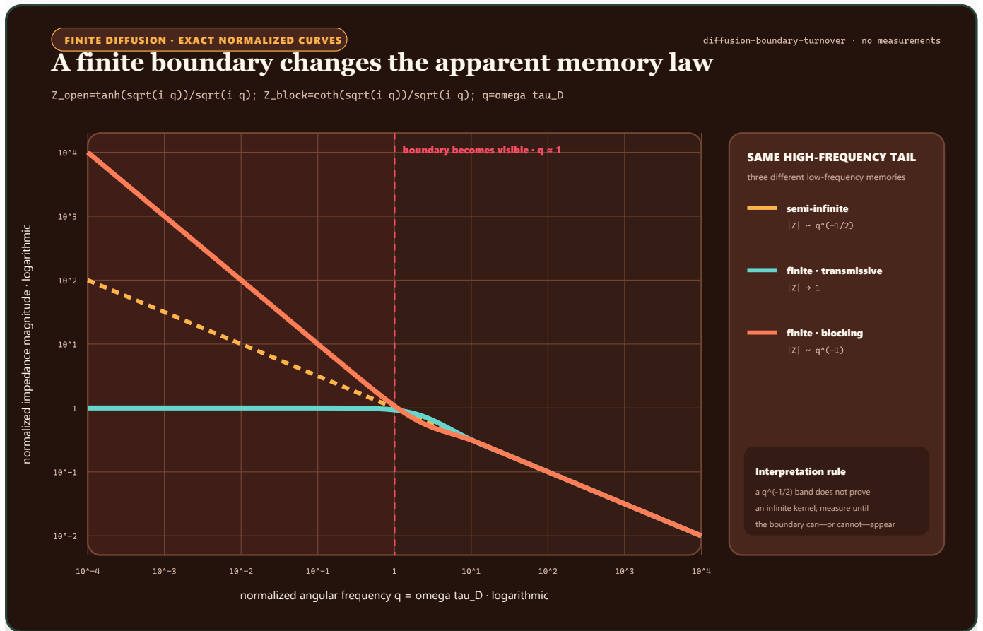
FIGURE 72 – A semi-infinite diffusion law and two finite-boundary laws coincide in their high-frequency slope but separate below the boundary timescale.
