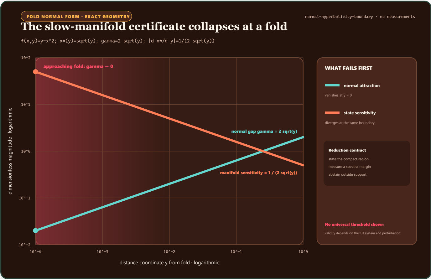
FIGURE 74 – In the fold normal form, the attracting spectral gap falls to zero while the slow-state sensitivity diverges.
