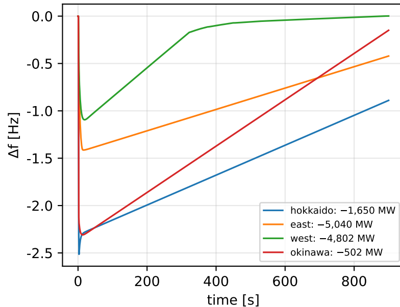
(b) largest online plant trip (upper-bound N-1, +UFLS)
