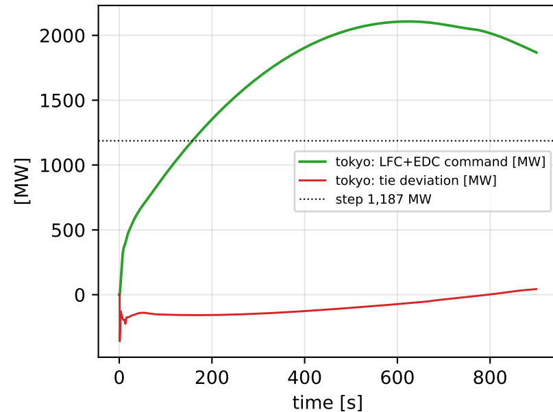
(c) TBC assigns correction to disturbed area
