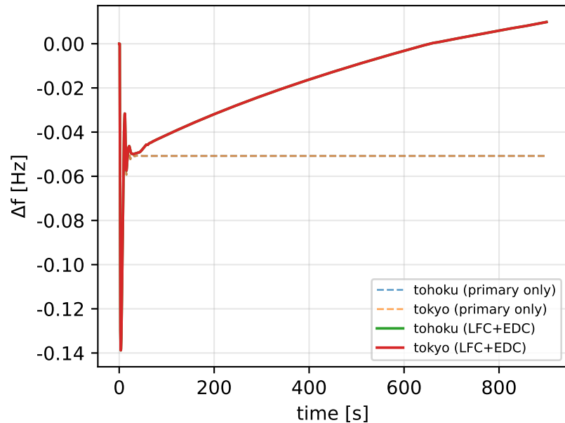
(a) east: 2% load step (1,187 MW)
