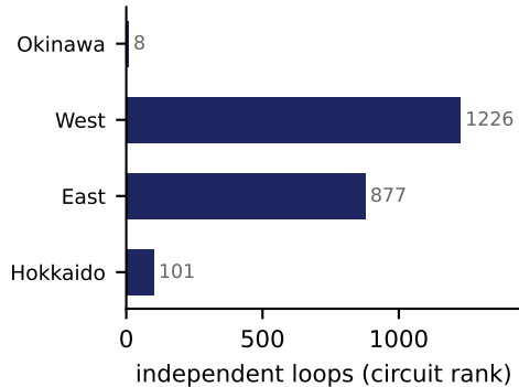
(a) Loops per synchronous island
