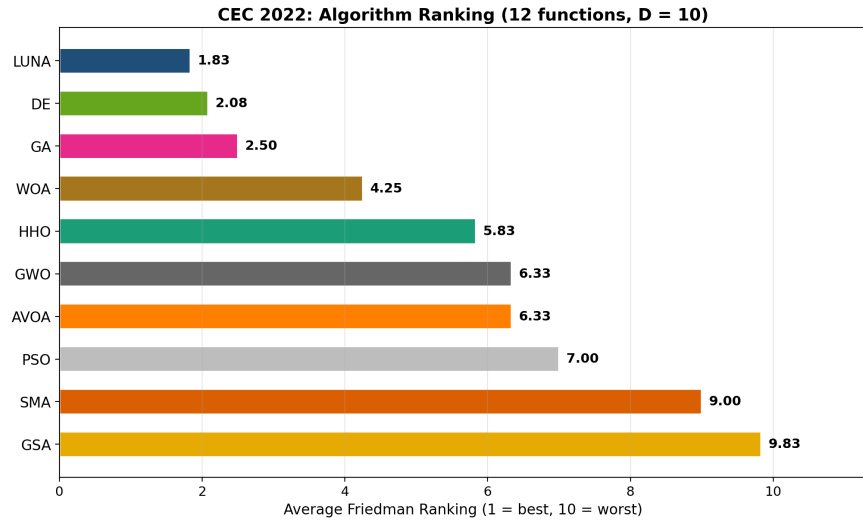
Figure 1: CEC 2022 Friedman ranking. LUNA ranks #1.
