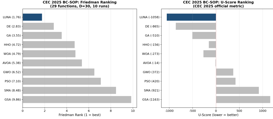
Figure 8: CEC 2025 BC-SOP results. Left: Friedman ranking (1 = best). Right: U-score (CEC 2025 official metric; lower = better). LUNA achieves rank #1 on both metrics, outperforming DE (rank 2.83) and GA (rank 3.55) by a substantial margin.
