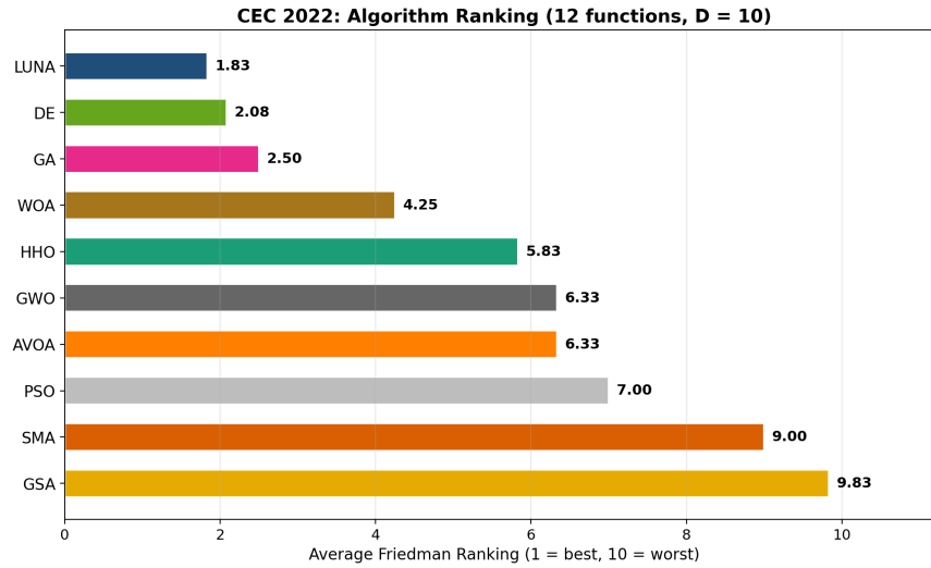
Figure 1: CEC 2022 Friedman ranking. LUNA ranks #1.
