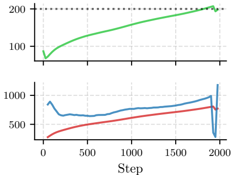
CNN \gamma = 0.02
