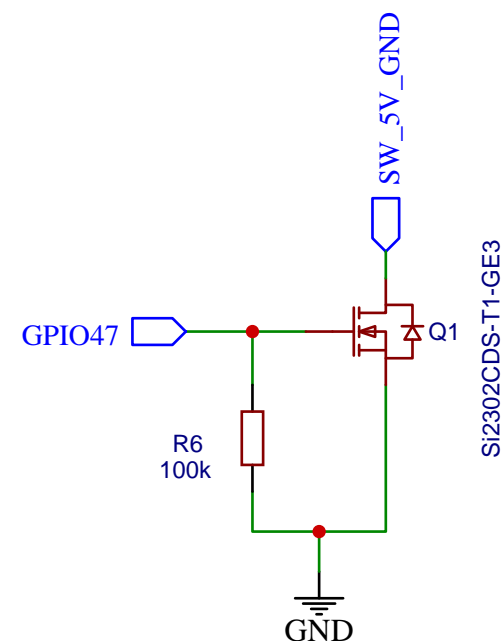
SWITCH for 1-Wire-Sensors
