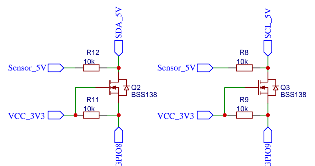
I2C Levelshifter 5V / 3.3V
