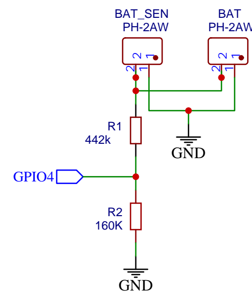
BATTERY SENSING
