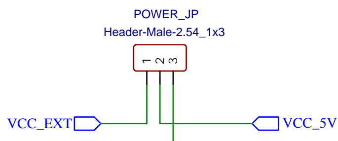
POWER SELECTOR
