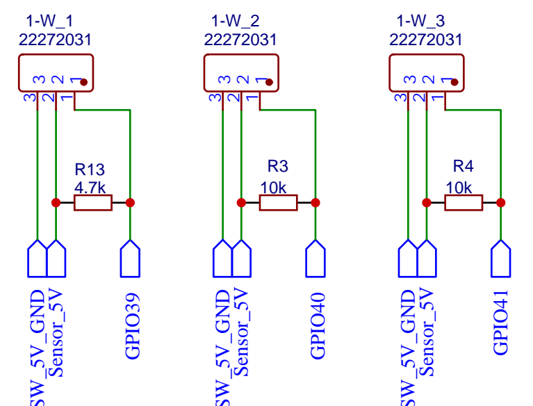
1-Wire-Sensor CONNECTORS
