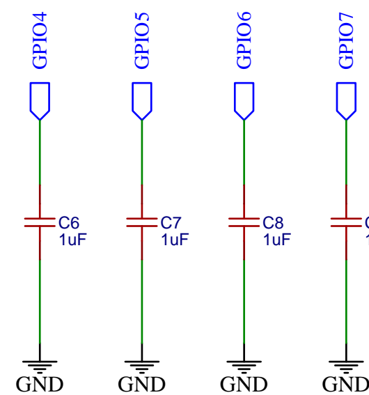
Analog Input Filter
