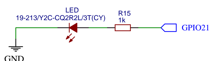
USER LED
