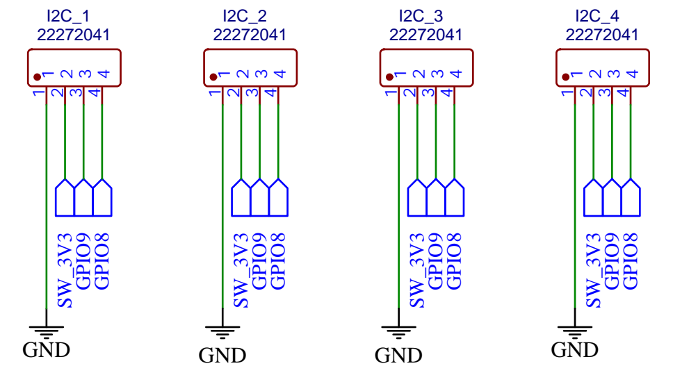
I2C SENSOR CONNECTORS
