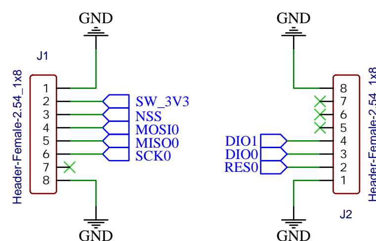
LoRA MODUL CONNECTOR
