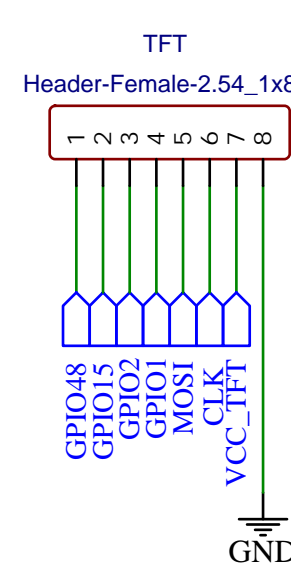
TFT CONNECTOR
