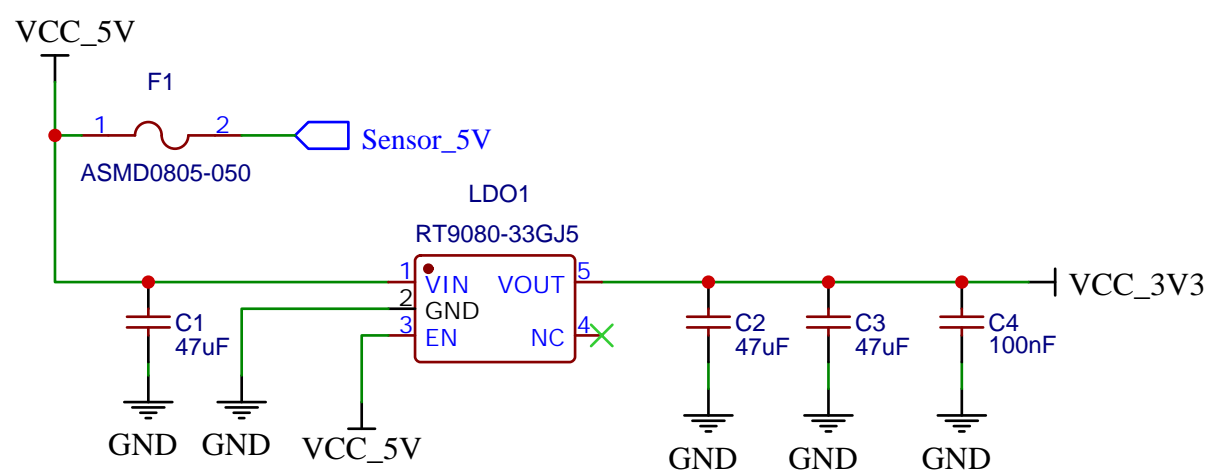
VOLTAGE REGULATOR 5V to 3.3V
